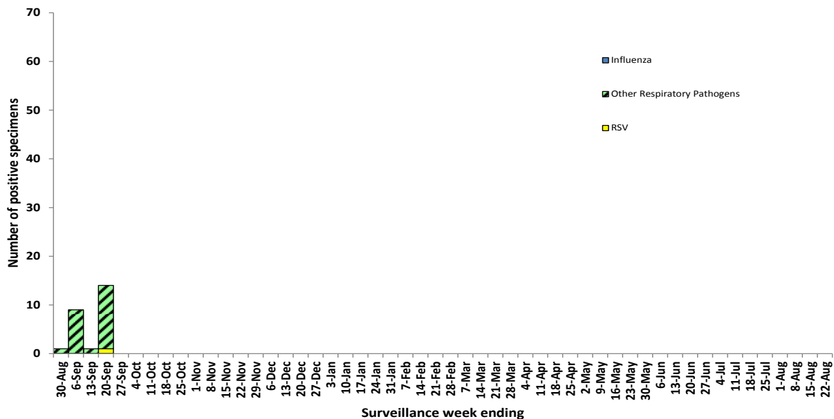
Figure 2: Summary of laboratory detected circulating respiratory pathogens, Nova Scotia, 2014–2015
