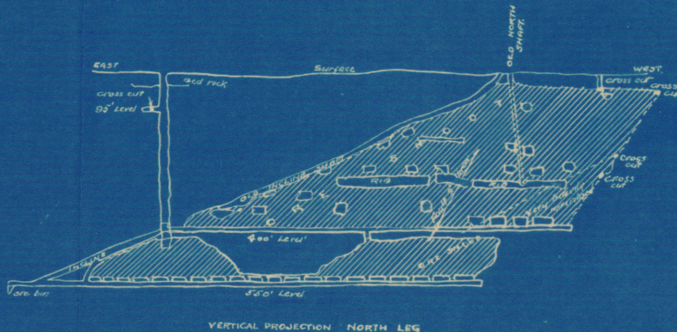
VERTICAL PROJECTION NORTH LEG
