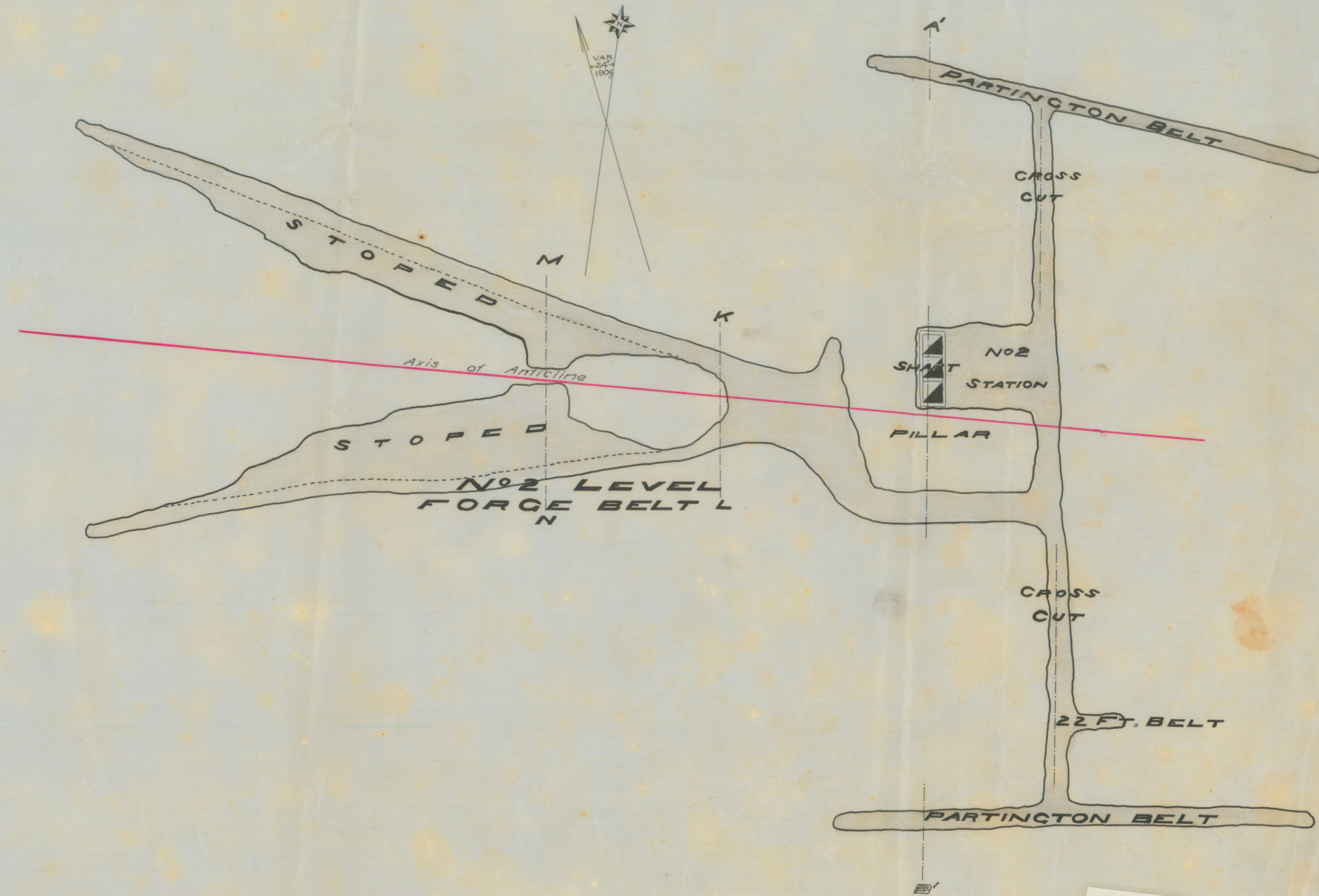
PLATE I HORIZONTAL PROJECTION OF WORKINGS ON LEVELS N°1 AND N°2
