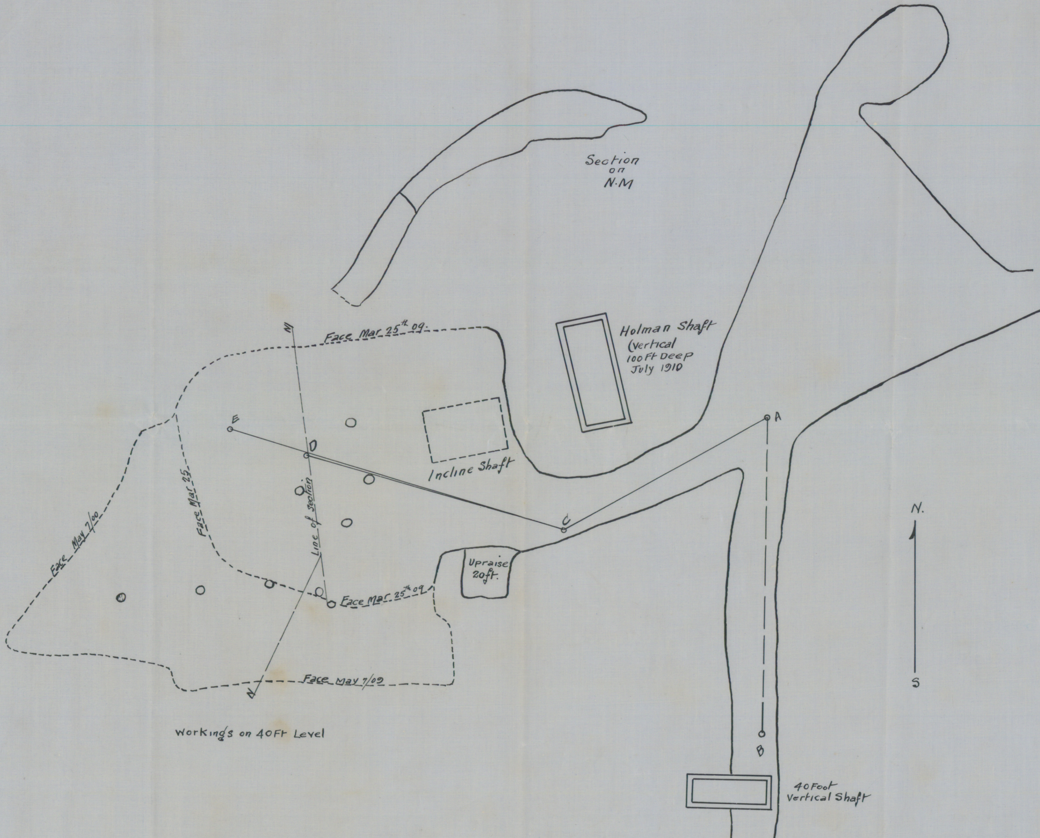
PLAN OF 40 FOOT LEVEL, HOLMAN GOLD MINE CARIBOU GOLD MINES.
