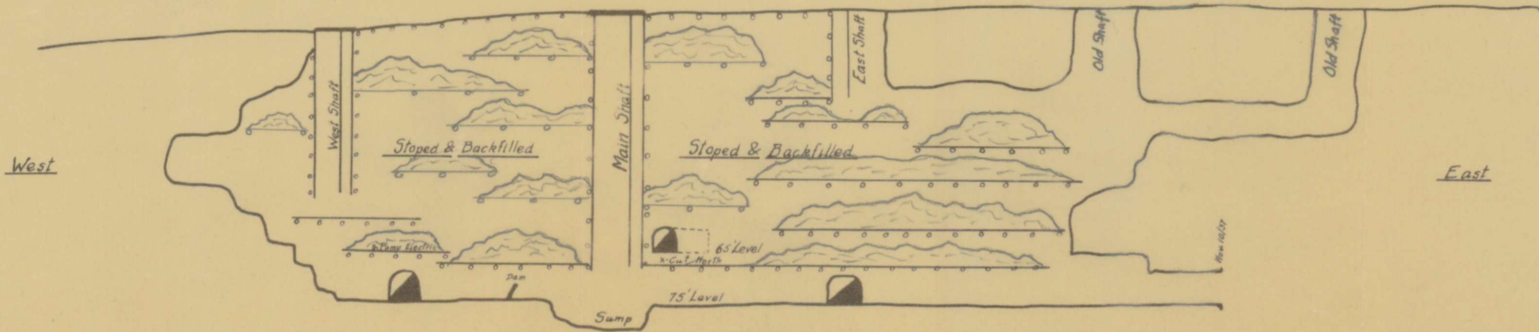
LONG. SECTION ON CAMERON VEIN
