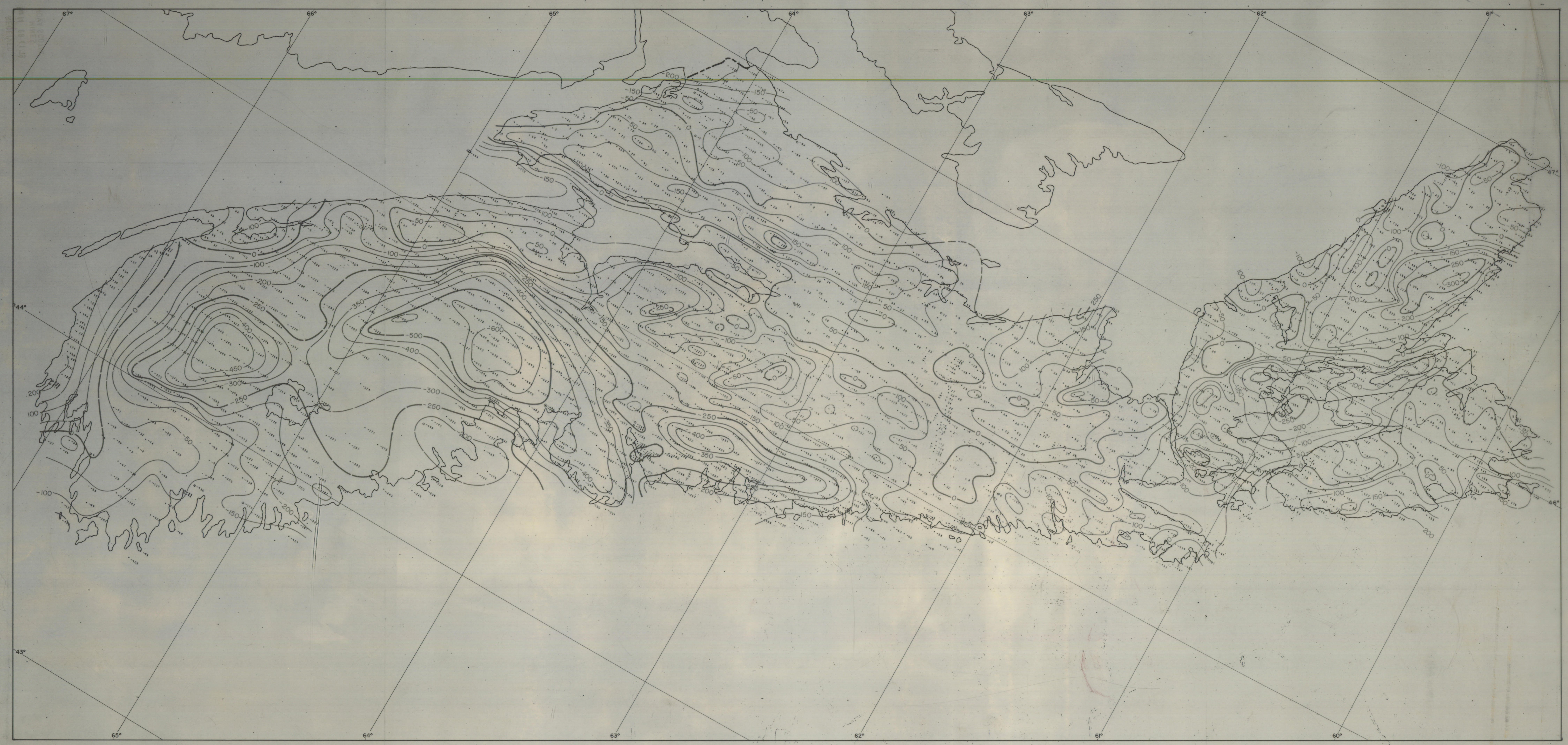
— BOUGUER ANOMALY MAP — Scale 1:500,000 Projection U.T.M.
