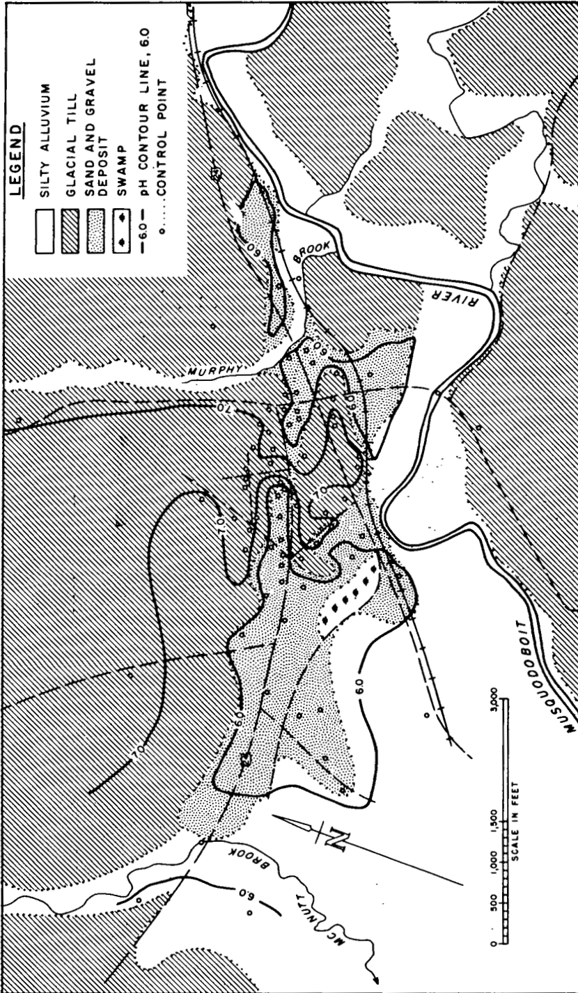
FIGURE 12. The pH values of groundwater in relation to the surficial geology at Middle Musquodoboit.
