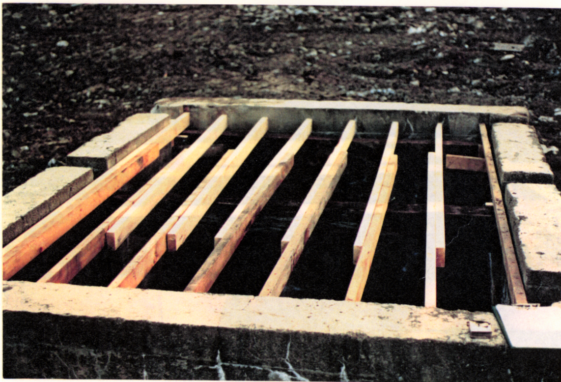
PHOTO NO. D-2: "Two by four" and railway tie timber support formwork for concrete cap.
