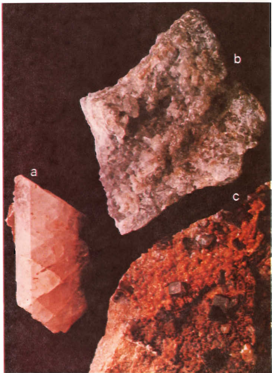
a. barite, North Greenville; b. celestite, Loch Lomond; c. fluorite in granite, Leminster.
