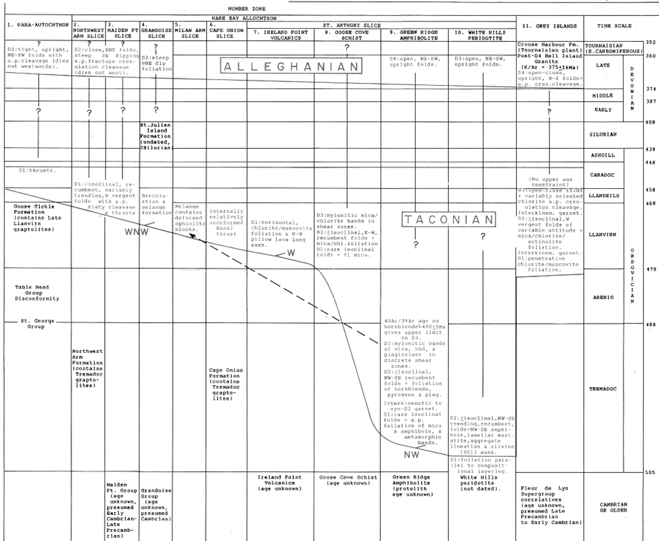
Figure 8. Correlation chart for structures in the Hare Bay transect, northernmost Newfoundland. References by column number: (1-6) Smyth, 1971; Williams, 1975; Stouge and Godfrey, 1982; Fahraeus, 1970; Stevens, 1970; Whittington and Kindie, 1963; Klappa et al., 1980; Erdtmann, 1971. (7-9) Smyth, 1971; Williams and Smyth, 1973; Girardeau, 1982; Crow, 1984; Jamieson, 1980; Dallmeyer, 1977. (10) Girardeau, 1982. (11) Kennedy et al., 1973.
