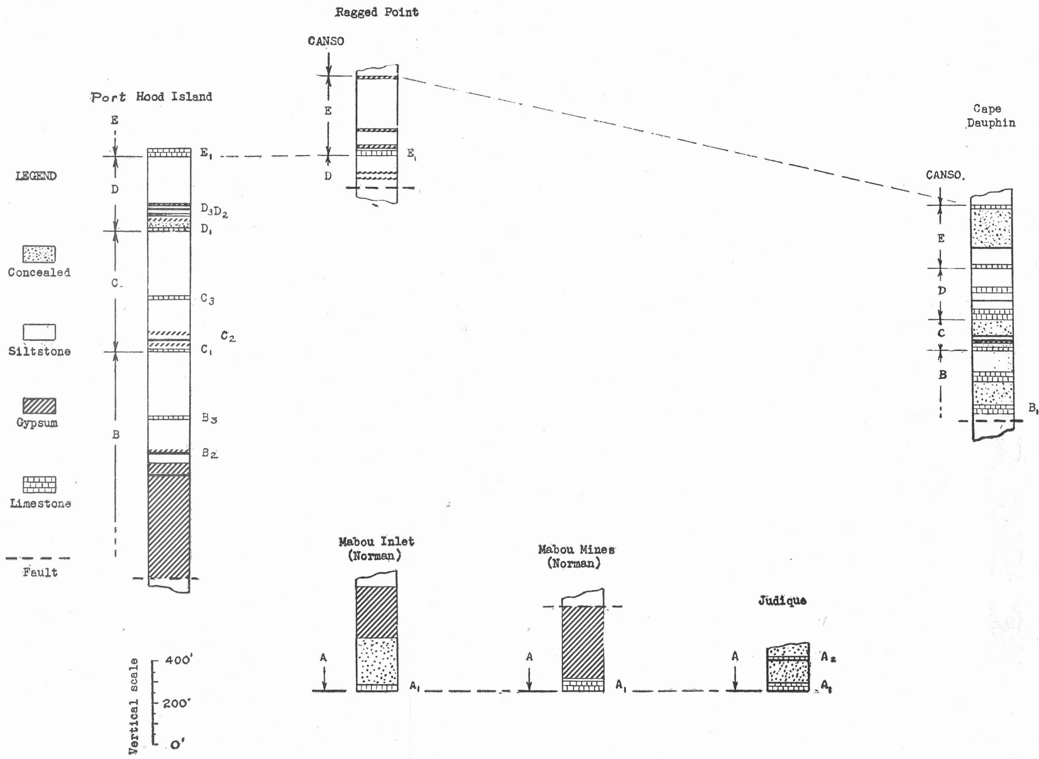
Fig. 3. Geologic Sections of the Windsor Group.
