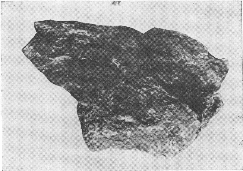
Figure 14. Typical algal structure ( \times\frac{1}{2} ) in the thin limestone members at the top of the E zone of the Windsor, and at the base of the Canso.
