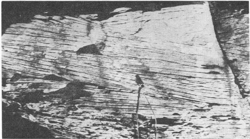
Figure 10. Typical lithology of the gray cross-bedded sandstones immediately below the Horton-Windsor contact.
