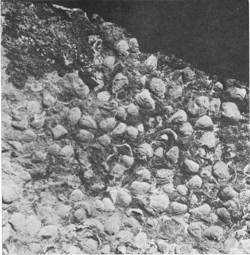
Figure 11. Weathered surface of the dolomite at the base of the E zone, loaded with Schizodus cf. S. denysi ; no other types of shells present.
