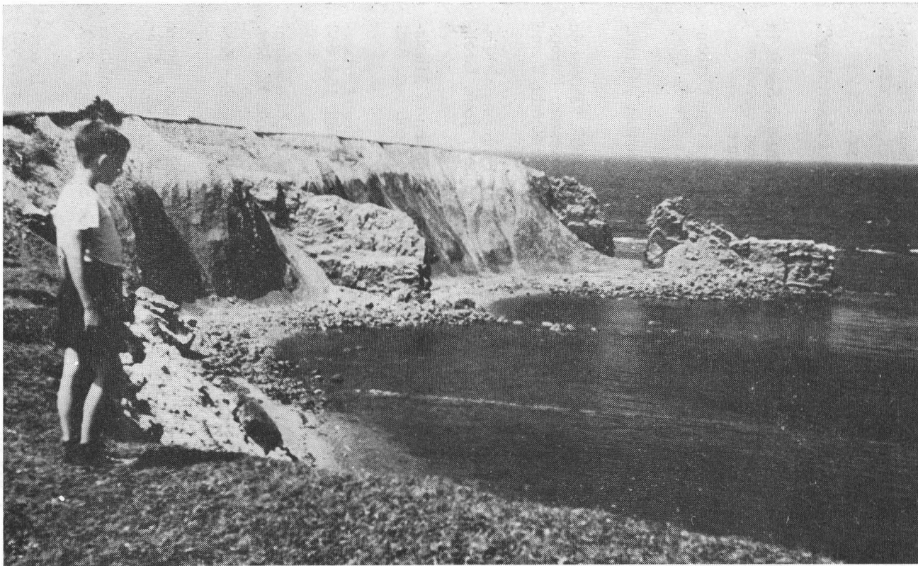
Figure 8. North shore of Port Hood Island, looking west toward Point Vertical, showing prominent exposures of limestones in the C and D zones. The camera is set up on the uppermost limestone in the B zone. Photo by courtesy of Professor Fairbairn.
