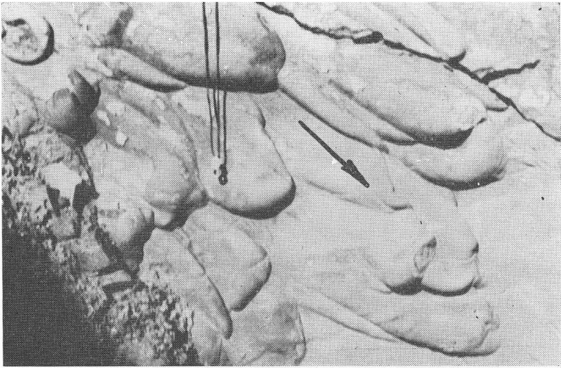
Figure 13. Flowcasts on base of Horton sandstone bed, near the Horton-Windsor contact, in the Southwest Mabou River. Hand lens gives scale. These are casts on the bottom of sandstones; the underlying mudstones have been removed. Arrow indicates direction of flow of water-filled sand.
