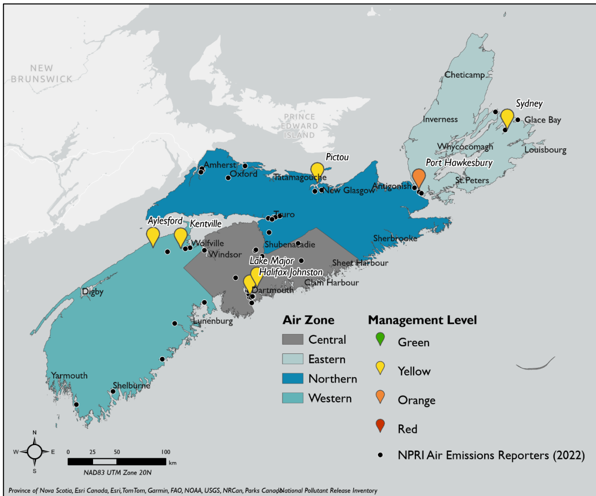
Figure 3. Nova Scotia's four air zones and the locations of ambient air monitoring stations. The station colour corresponds to the management level achieved at that station in 2022.
