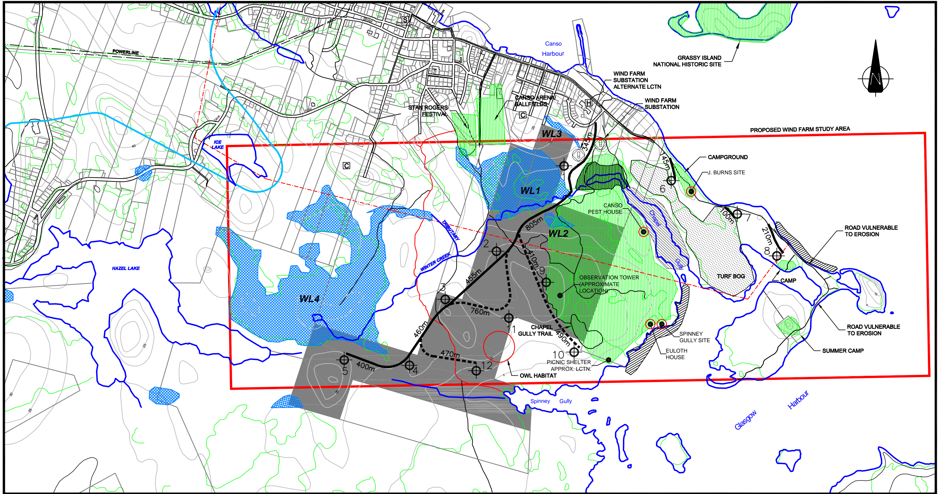
FIGURE 2.3 ENVIRONMENTAL AND CONSTRUCTION CONSTRAINTS SCALE 1:15000 PROPOSED CANSO WIND FARM CANSO, NS
