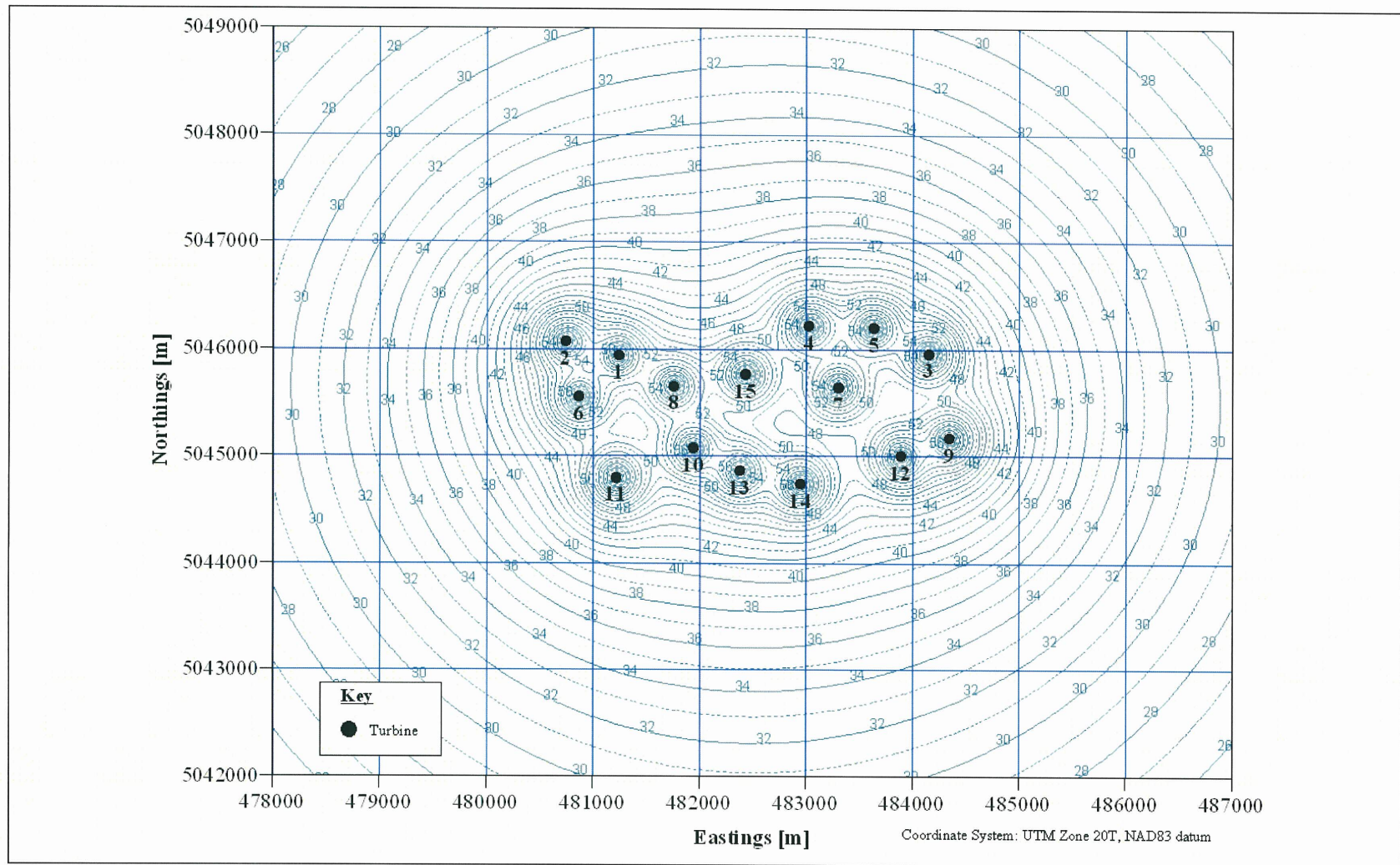
Figure 2 Predicted noise mapping at the Nuttby Wind Farm Layout 1 at 8 m/s at 2 m.
