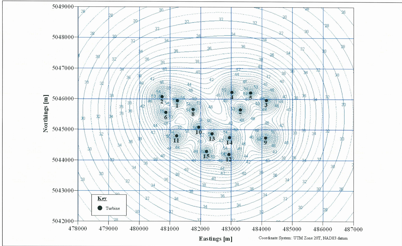
Figure 4 Predicted noise mapping at the Nuttby Wind Farm Layout 2 at 8 m/s at 2 m.
