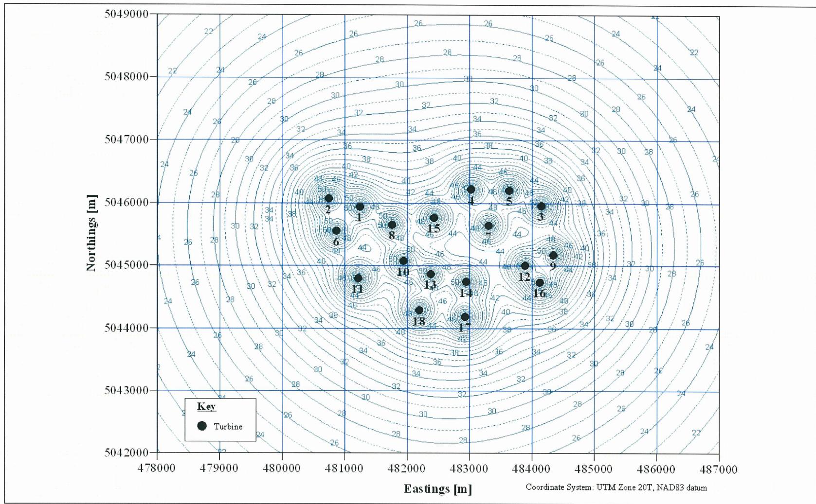
Figure 6 Predicted noise mapping at the Nuttby Wind Farm Layout 3 at 8 m/s at 2 m.
