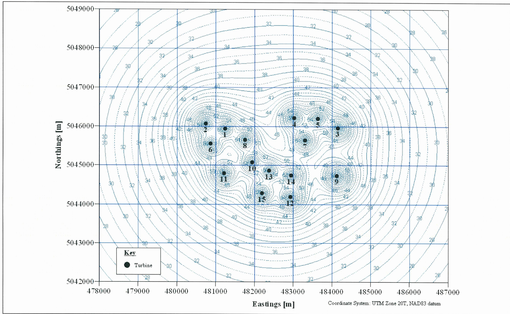
Figure 3 Predicted noise mapping at the Nuttby Wind Farm Layout 2 at 6 m/s at 2 m.
