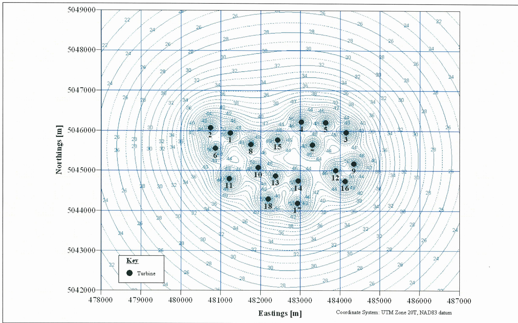
Figure 5 Predicted noise mapping at the Nuttby Wind Farm Layout 3 at 6 m/s at 2 m.
