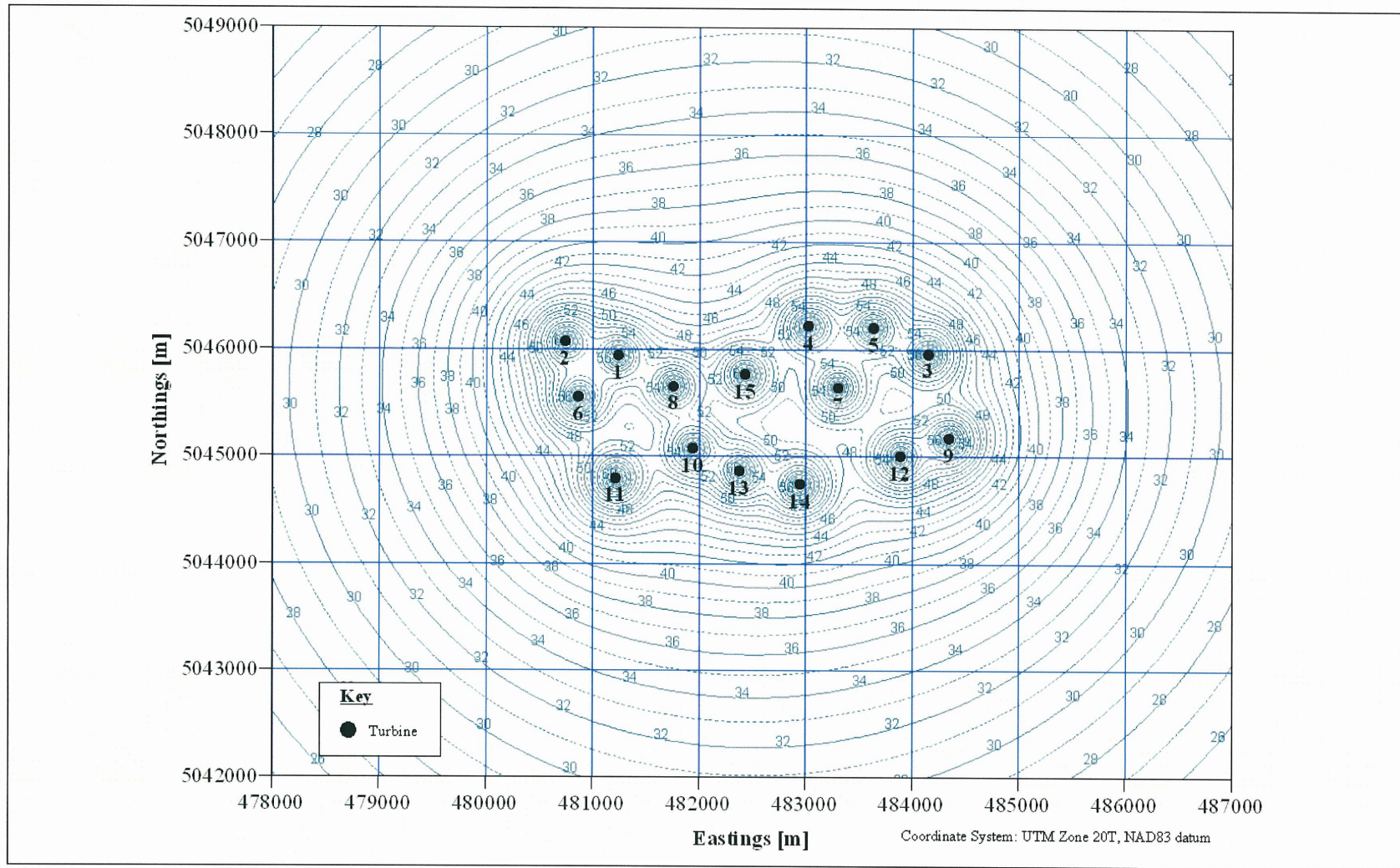
Figure 1 Predicted noise mapping at the Nuttby Wind Farm Layout 1 at 6 m/s at 2 m.
