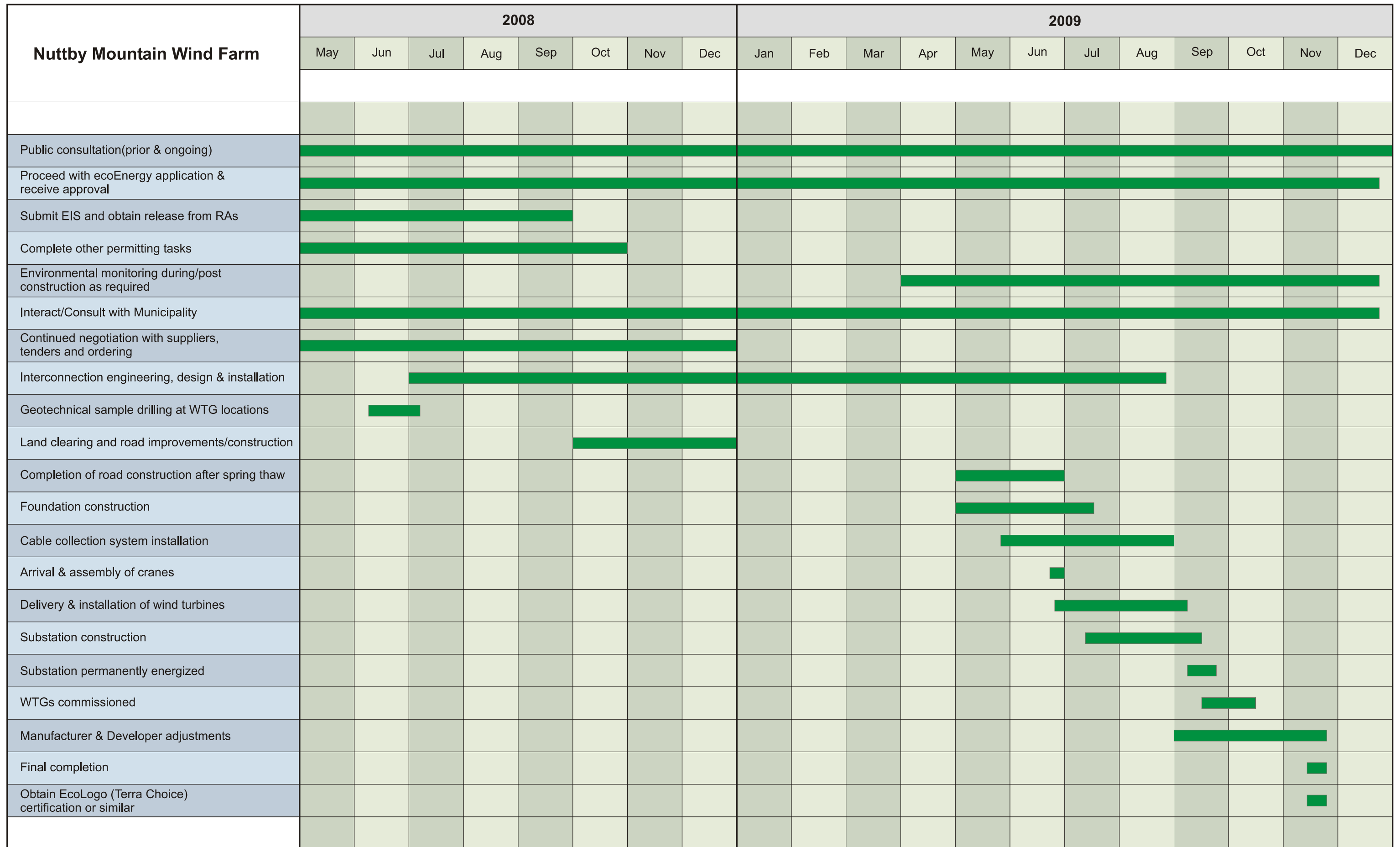
FIGURE 2.5:Project Schedule
