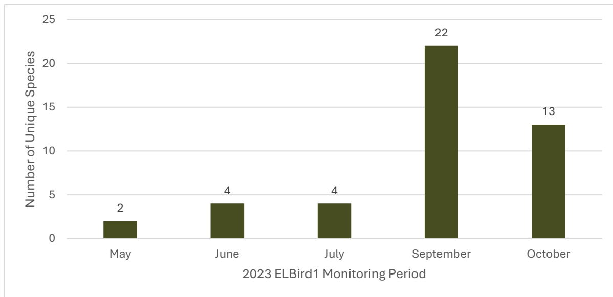
Figure 3.5: Nighthawk Species Richness during the 2023 Monitoring Period at ELBird1
