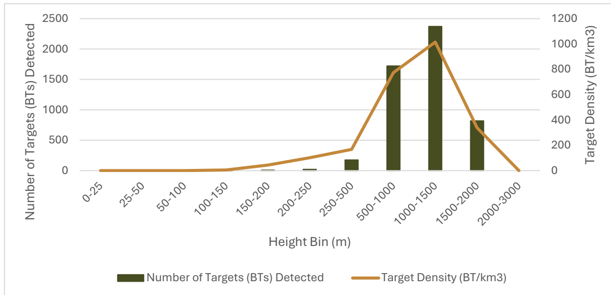
Figure 2.11: Target Height and Target Density – Fall 2023
