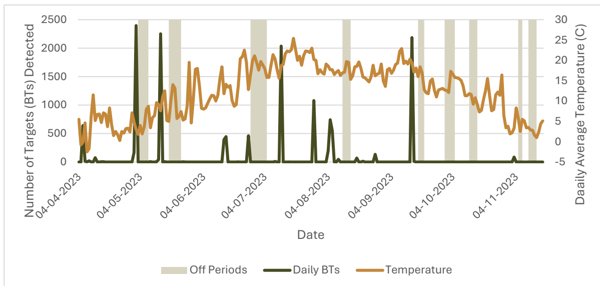
Figure 2.7: Number of Biological Targets Detected during the 2023 ARS Fall Monitoring Period Compared to Daily Mean Temperature (°C)
