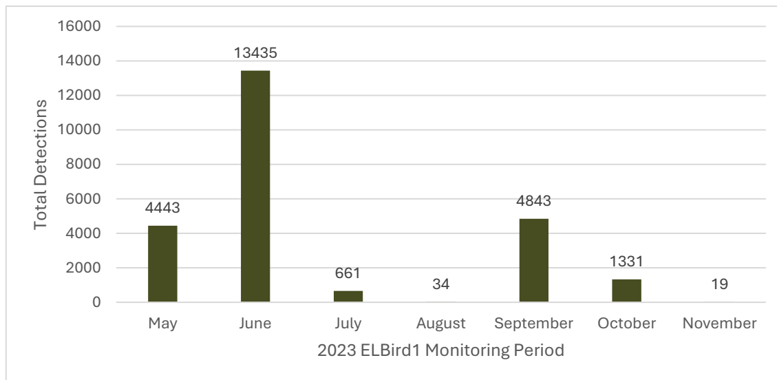
Figure 3.1: Detections made by Nighthawk at ELBird1 during the 2023 Monitoring Period
