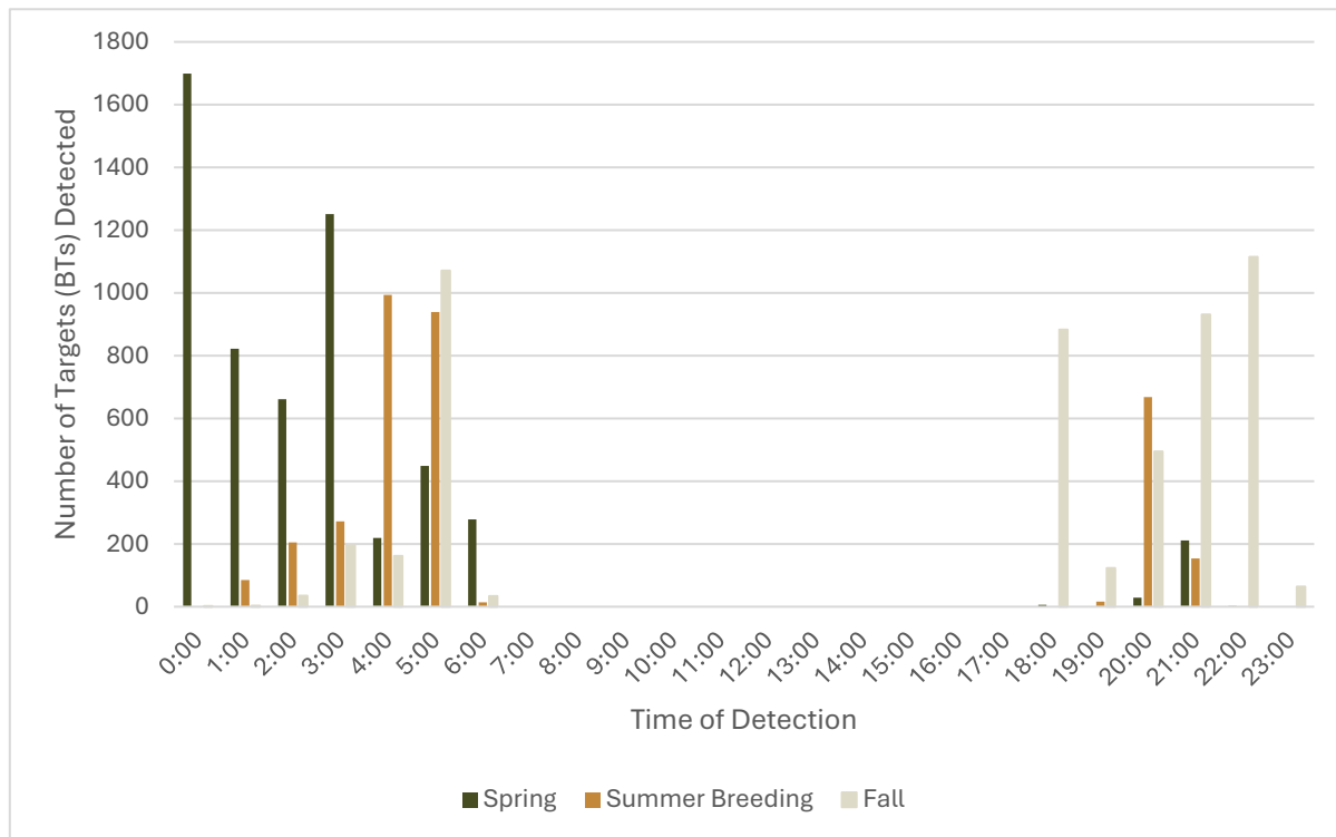
Figure 2.4: Number of BTs Detected per hour throughout the 2025 Monitoring Period
