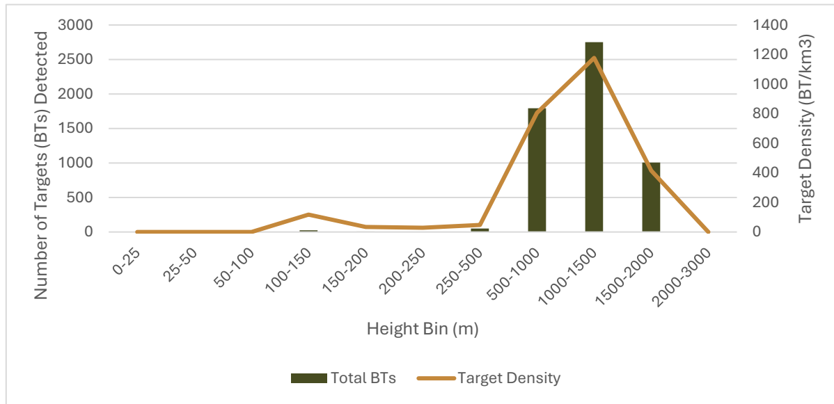
Figure 2.9: Target Height and Target Density – Spring 2023
