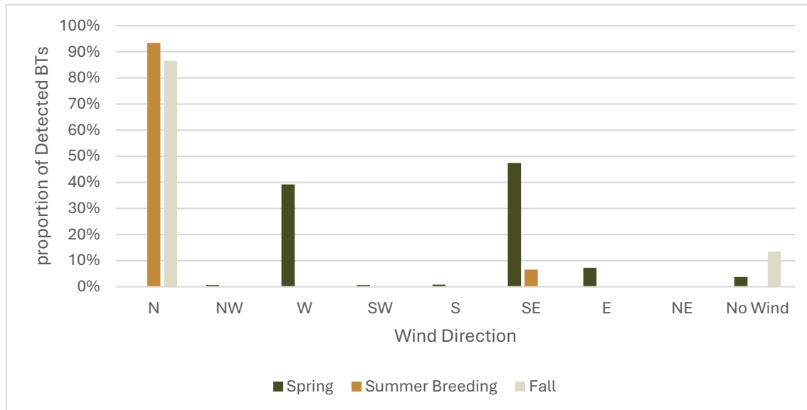
Figure 2.5: Wind Direction by Proportion of BTs Detected - 2023
