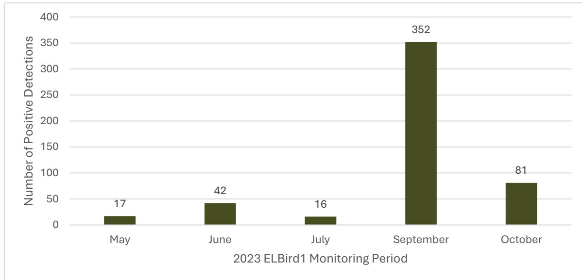
Figure 3.3: Positive Nighthawk detections at ELBird1 during the 2023 Monitoring Period
