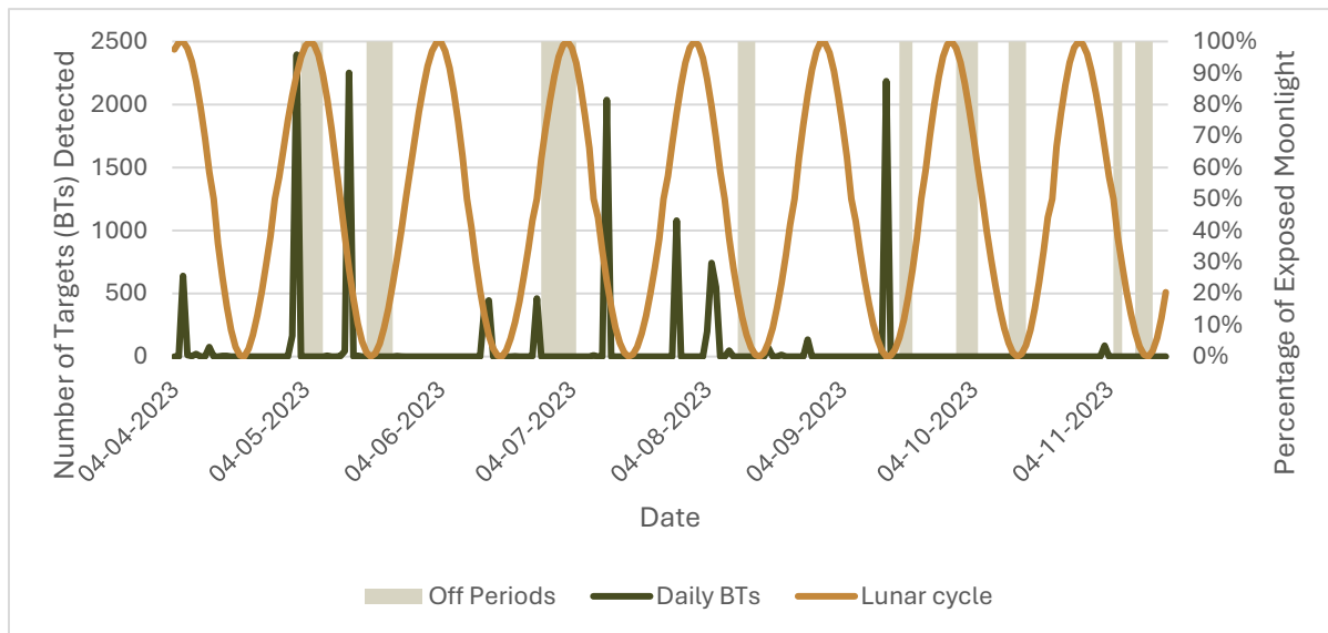
Figure 2.8: Number of Biological Targets Detected during the 2023 ARS Monitoring Period Compared to Lunar Cycle
