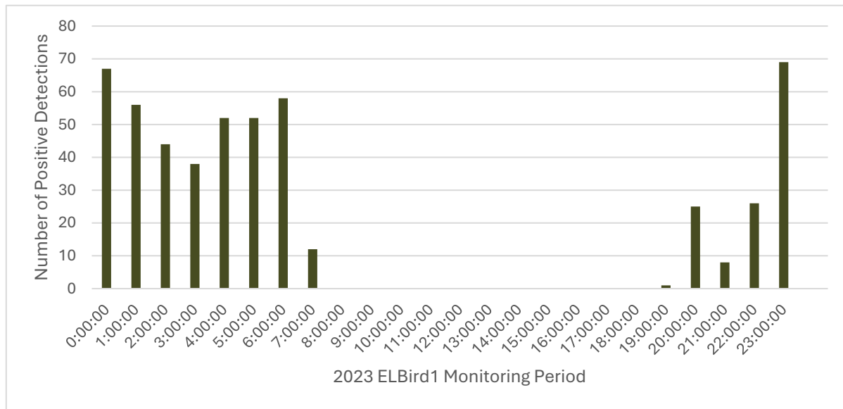
Figure 3.4: Timeframe of Positive Nighthawk Detections at ELBird1 during the 2023 Monitoring Period
