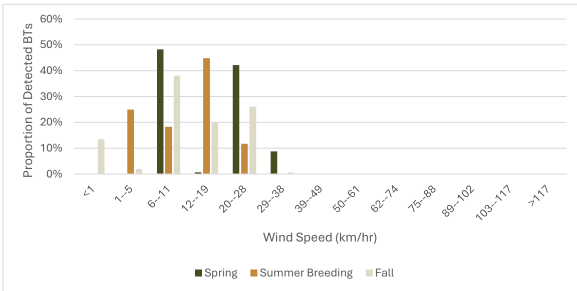
Figure 2.6: Wind Speed by Proportion of BTs Detected - 2023
