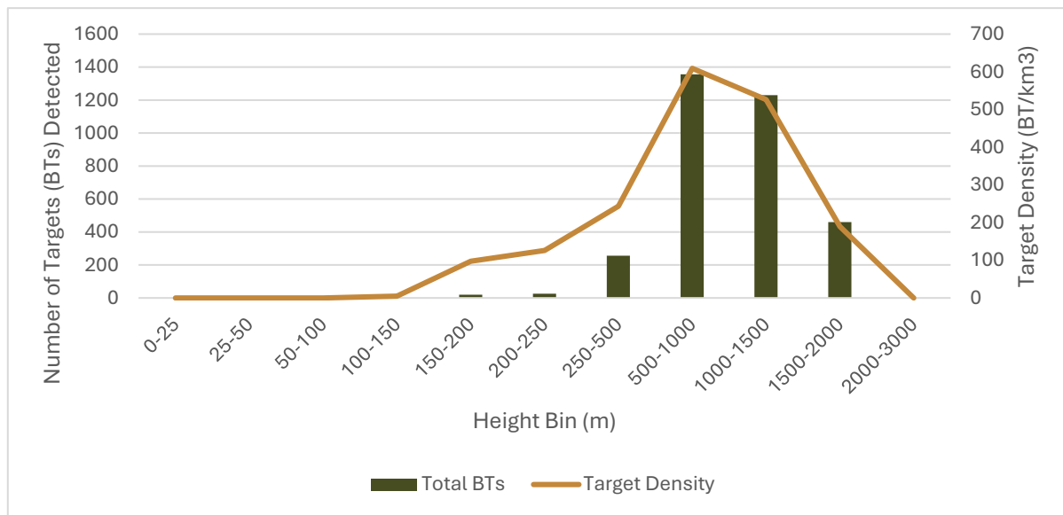
Figure 2.10: Target Height and Target Density – Summer Breeding 2023
