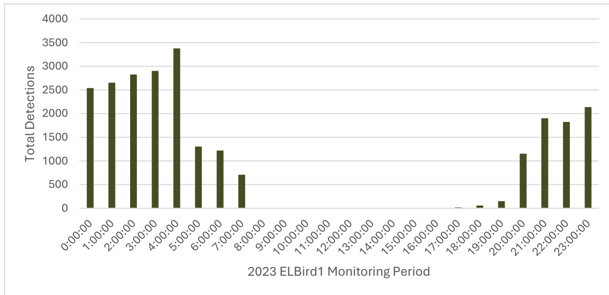
Figure 3.2: Timeframe of Nighthawk Detections at ELBird1 during the 2023 Monitoring Period
