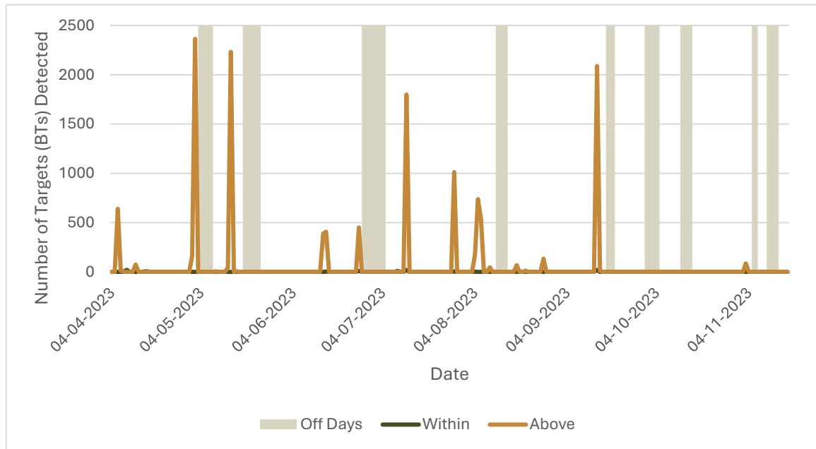
Figure 2.12: Number of Detections Within or Above the Rotor Swept Area During the 2023 ARS Monitoring Campaign
