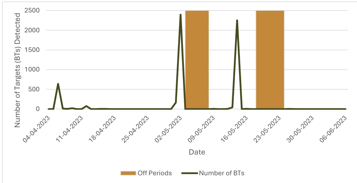
Figure 2.1: Number of BTs detected throughout the 2023 Spring Monitoring Period
