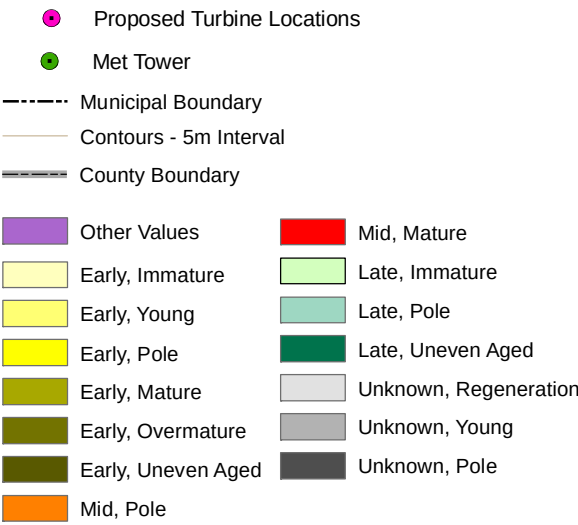
Figure 4.2 Regional Forest Cover Seral Stage & Maturity
