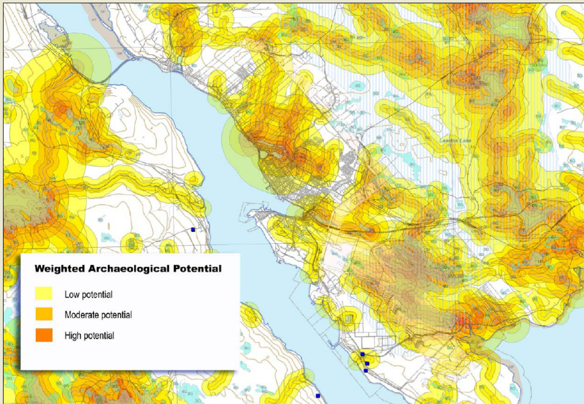
FIGURE 4.5: Weighted Archaeological Potential for First Nation Sites
