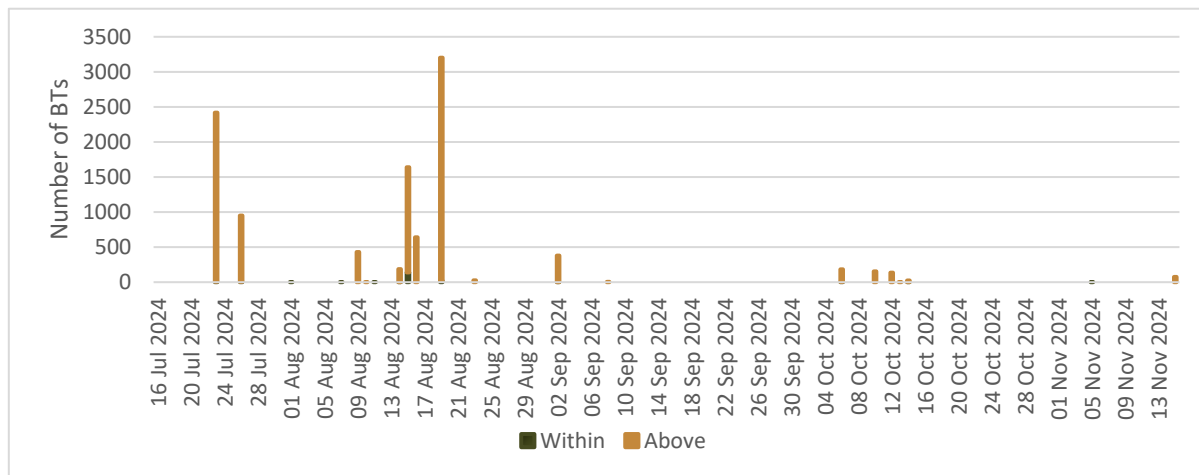
Figure 3.8: Number of Detections Within or Above the Rotor Swept Zone During the Fall 2024 Monitoring Period
