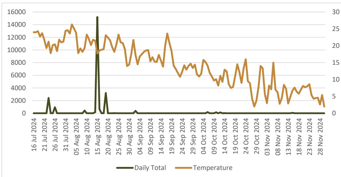
Figure 3.5: Number of Biological Targets Detected during the 2024 ARS Fall Monitoring Period Compared to Daily Mean Temperature (°C)
