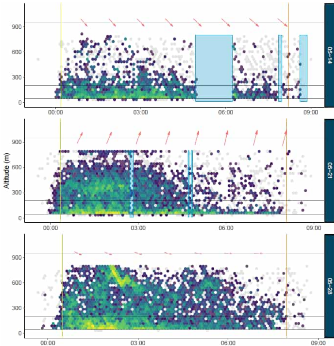
Figure 3.2 Targets Detected by Radar on April 28 and 30, and May 8, 12, 14, 21 and 28, 2023.
