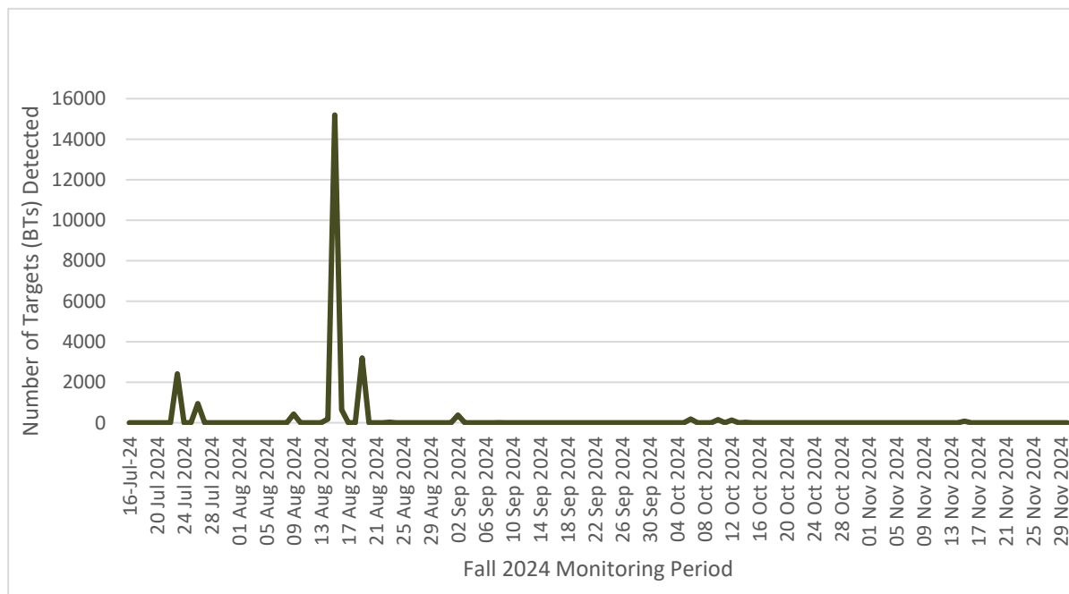
Figure 3.1: Number of BTs detected throughout the 2024 Fall Monitoring Period
