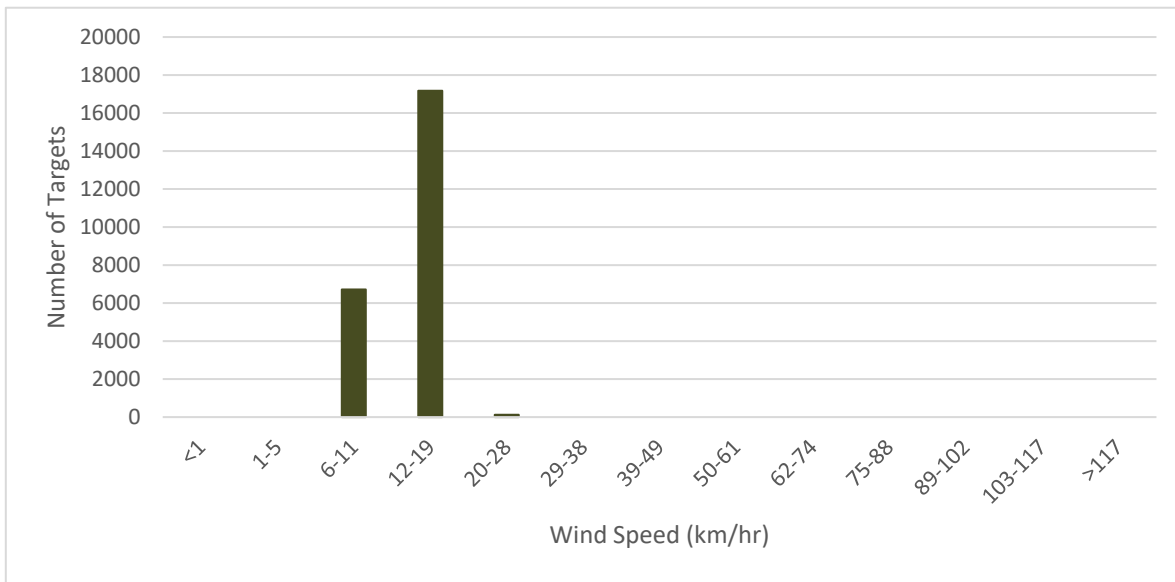
Figure 3.4: Wind Speed by Proportion of BTs Detected - Fall 2024
