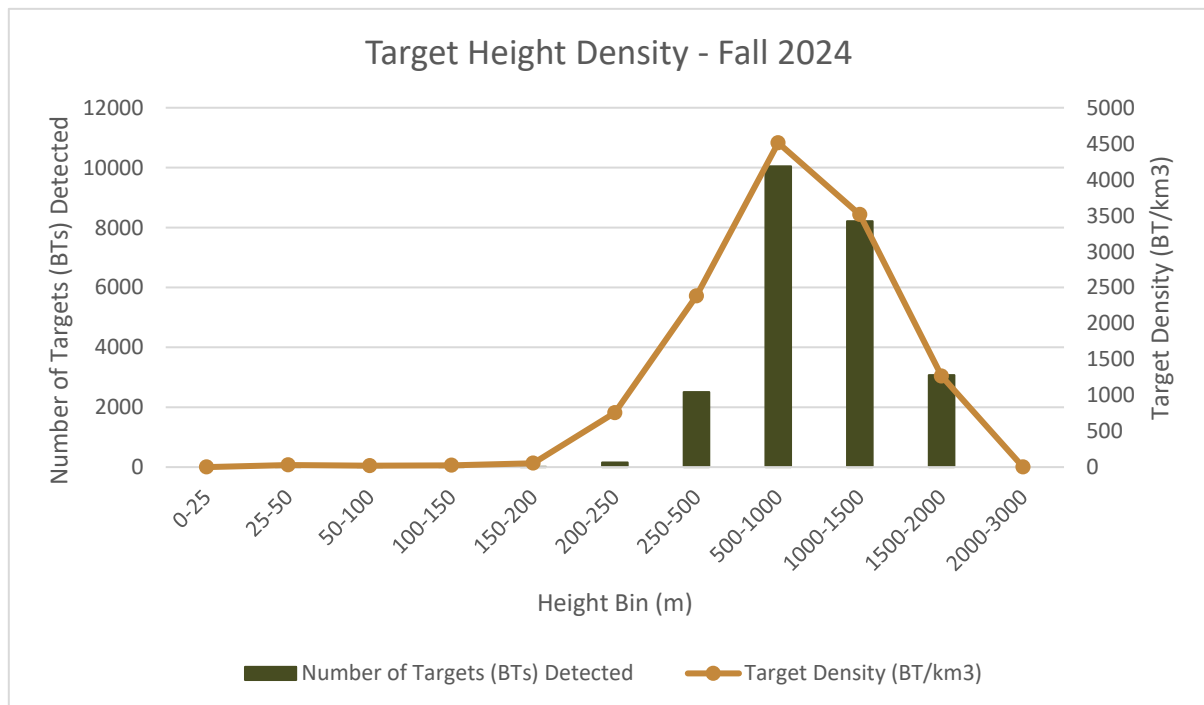
Figure 3.7: Target Height and Target Density – Fall 2024
