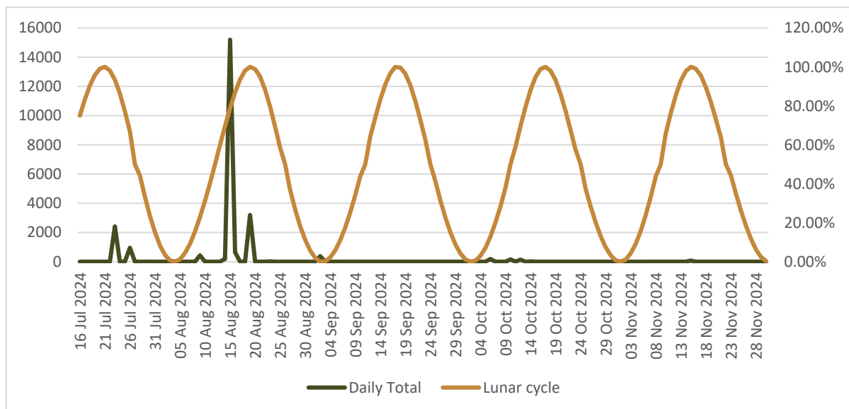
Figure 3.6: Number of Biological Targets Detected during the 2024 ARS Fall Monitoring Period Compared to Lunar Cycle
