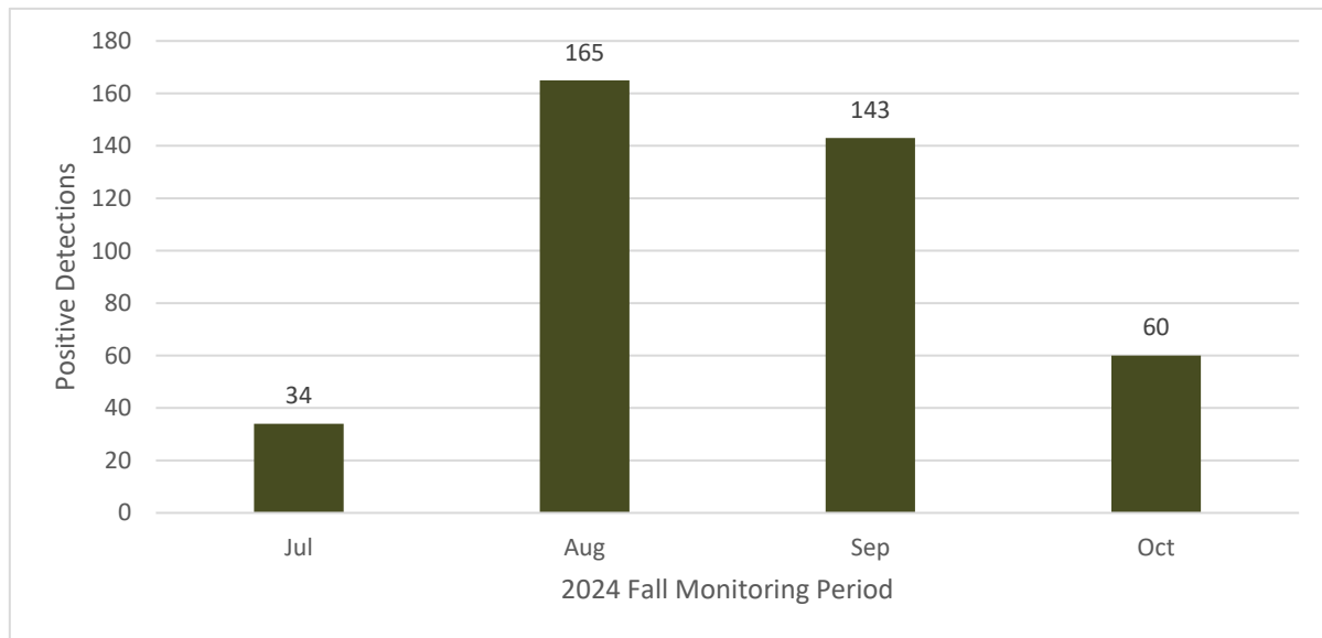
Figure 3.14: Positive Nighthawk Detections at ARU3 during the 2024 Fall Monitoring Period
