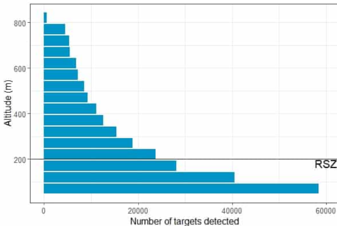
Figure 3.3 Altitudinal Profile of Targets Detected in Spring 2023.
