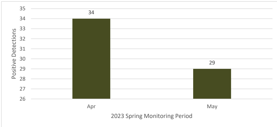
Figure 3.10: Positive Nighthawk Detections for ARU3 during the 2023 Spring Monitoring Period
