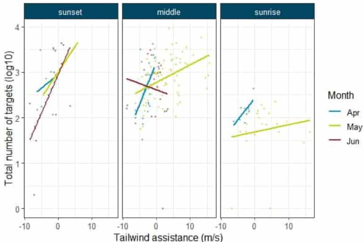
Figure 3.5 Relationship between Tailwind Assistance and the Total Number of Targets across Time of Night and Season during Spring 2023.
