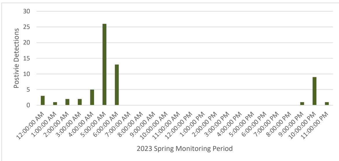
Figure 3.11: Timeframe of Positive Nighthawk Detections at ARU3 during the 2023 Spring Monitoring Period
