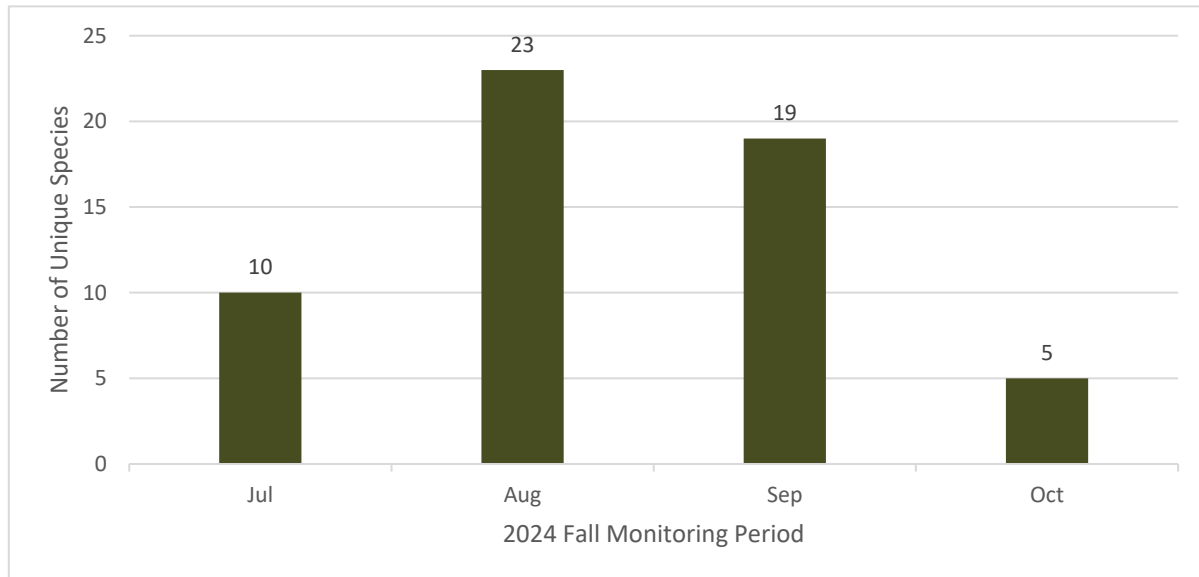
Figure 3.16: Nighthawk Species Richness at ARU3 during the 2024 Fall Monitoring Period
