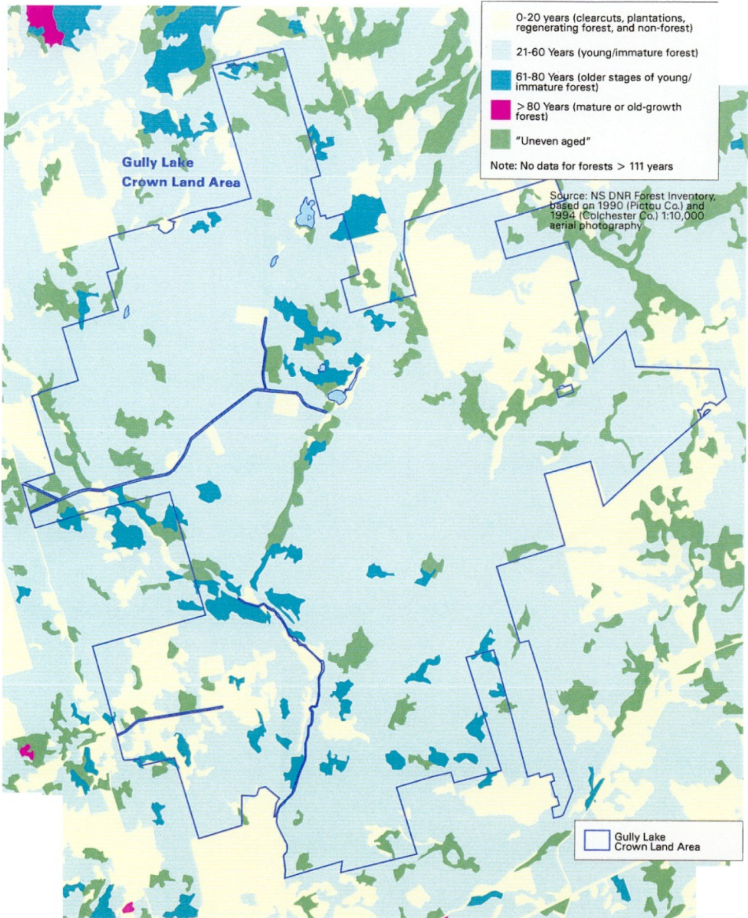
Map 5. Forest Age Classes in the Gully Lake Crown Land Area.
