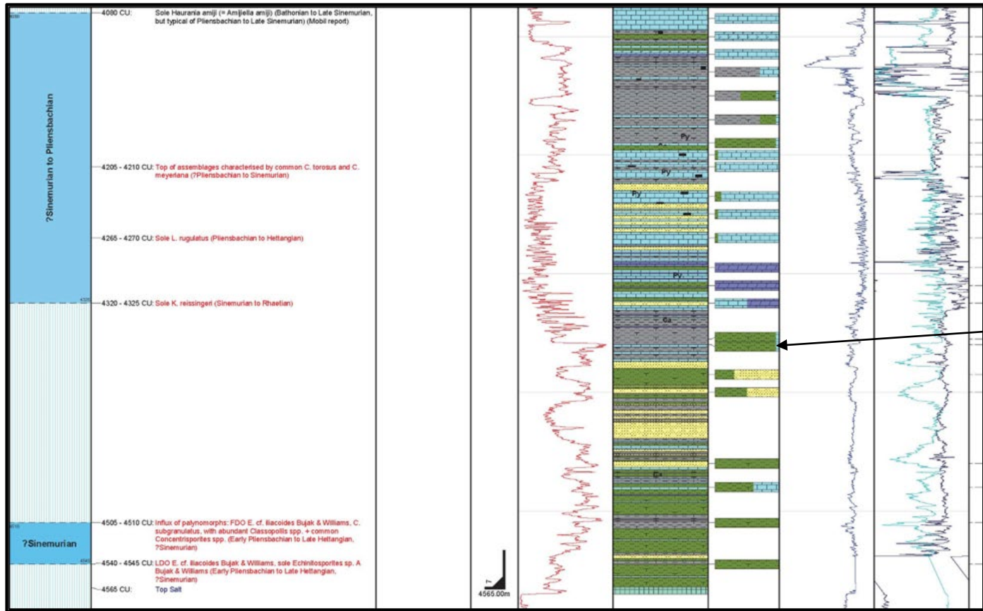
Figure 14: Snapshot of the Cap Juby-1 ST4 Stratigraphic Summary Log showing age determinations and the position of black siltstones (?source facies).
