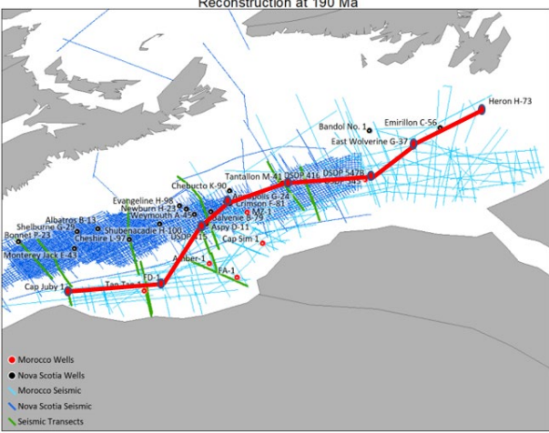
Figure 12: Chronostratigraphic Chart of Cretaceous strata in wells studied across the Scotian-Moroccan conjugate margins. Well locations shown above, with red line indicating locations on the reconstruction of the margins at 190 Ma (Pliensbachian). Timescale of Chronostratigraphic Chart: Ogg, Ogg & Gradstein (2016).
