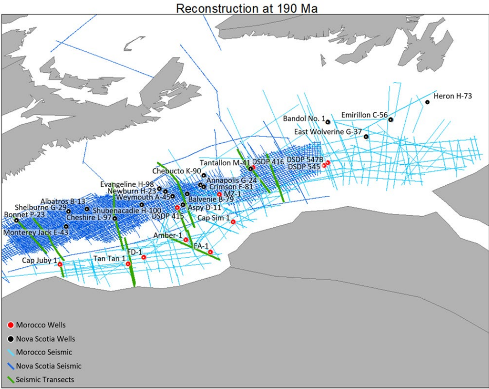
Figure 10: Reconstruction of the Scotian and the conjugate Moroccan margins at 190 Ma (Pliensbachian) showing wells studied from the Scotian Margin (black dots) and from the Moroccan Margin (red dots). Reconstructed seismic transects from the Beicip-Franlab Atlas (2019) are shown in green.
