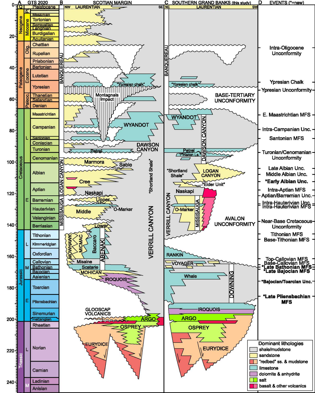
Figure 2: Wheeler Diagram showing lithostratigraphy (B and C) and biostratigraphic events (D) on the Scotian Margin (B) in comparison to the southern Grand Banks area (C) (Weston et al. , 2023). Scotian Margin chart is modified from Weston et al. (2012) and Deptuck and Altheim (2018); it does not show post-depositional salt tectonic movement. Grand Banks chart is modified from Sinclair (1988), McAlpine (1990) and MacLean and Wade (1992). Age of volcanic rocks is based on Pe-Piper and Jansa (1987) and Bowman et al. (2012). Timescale (A) is from Gradstein et al. (2020). Two colour shades for 'redbeds' refer to sandstone- and mudstone-dominated lithologies, respectively, and the two shades for volcanic rocks refer to basalts and other types of volcanic rocks, respectively. Formation labels are in upper case, members are lower case. Informal units are in quotation marks. Abbreviations: ls. = limestone; ss. = sandstone; Unc. = unconformity; MFS = maximum flooding surface; Pl. = Pliocene; Olig. = Oligocene; Paleoc. = Paleocene; E. = Early; M. = Middle; L. = Late.
