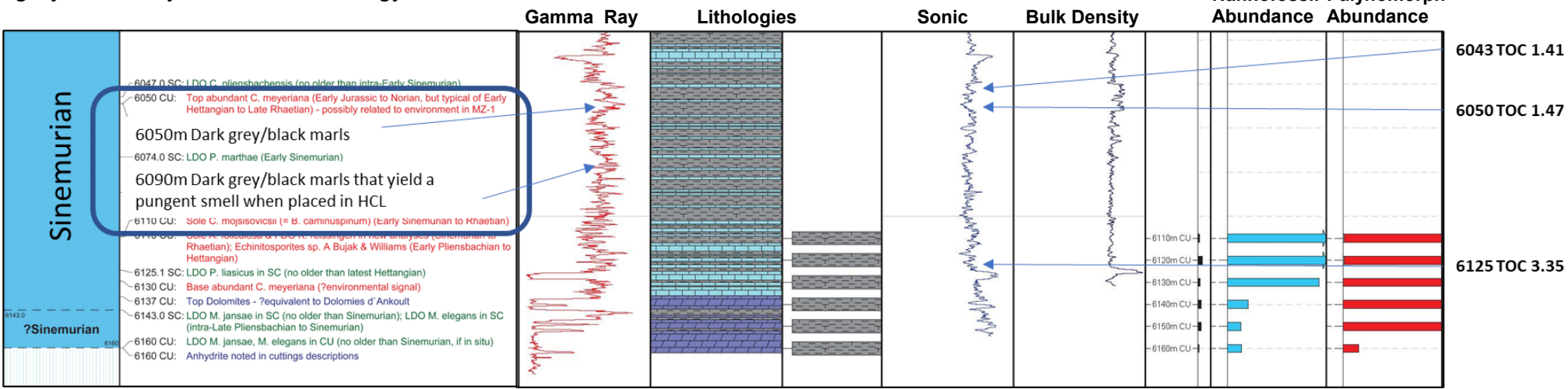
Figure 13: Snapshot of the MZ-1 Stratigraphic Summary Log showing the deepest part of the well above TD at 6160m. Note the thin dark/grey/black marls (?source facies) at 6050m and 6090m in strata dated as Early Sinemurian.
