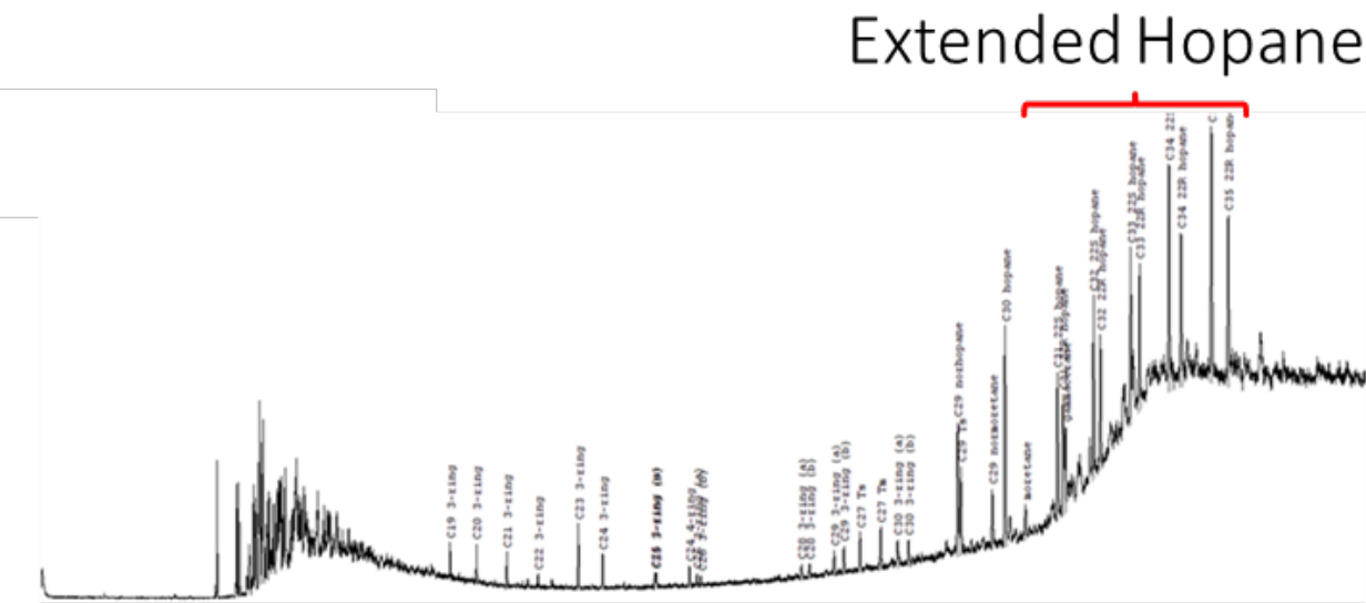
Figure 20: Mic Mac J-77 saturate GCMS (m/z 191) showing the extended hopane biomarkers (Fowler, 2020).
