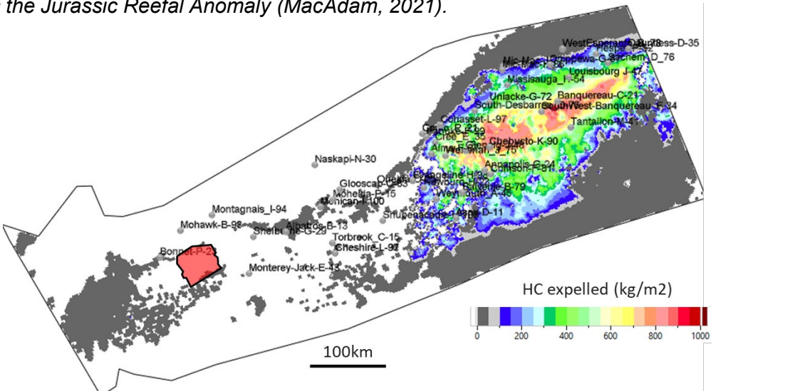
Figure 28: Tithonian hydrocarbon expulsion map showing this source rock has not expelled any hydrocarbons in the area of the anomaly.
