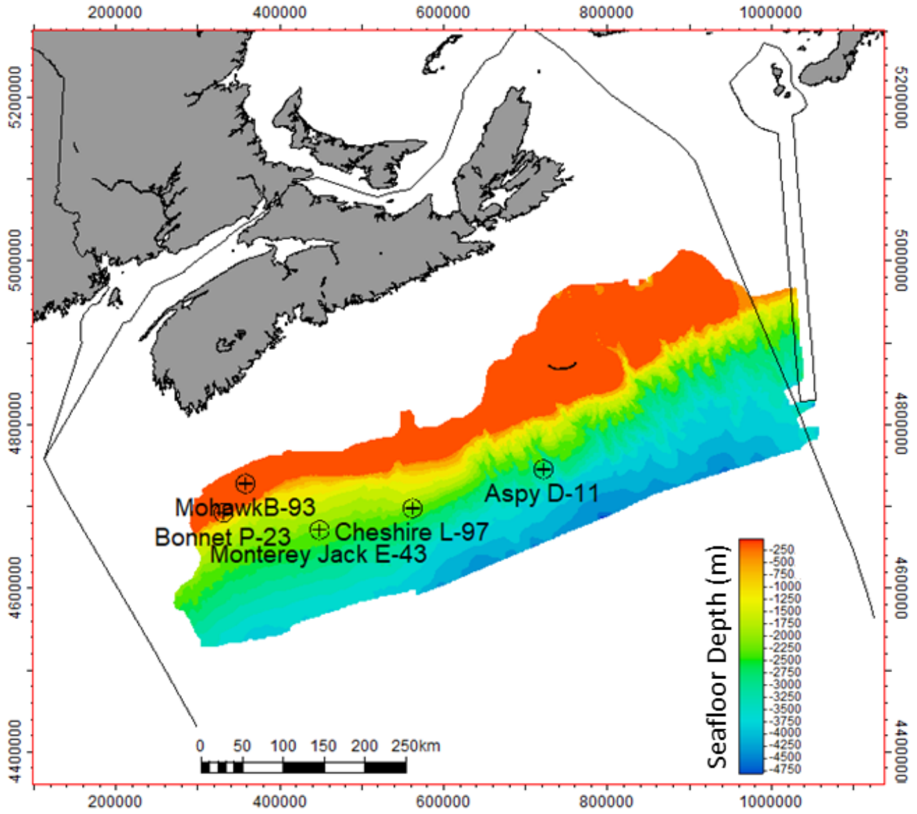
Figure 61: Location of the Barrington 3D survey, wells used in the study, and extent of the legacy basin model.
