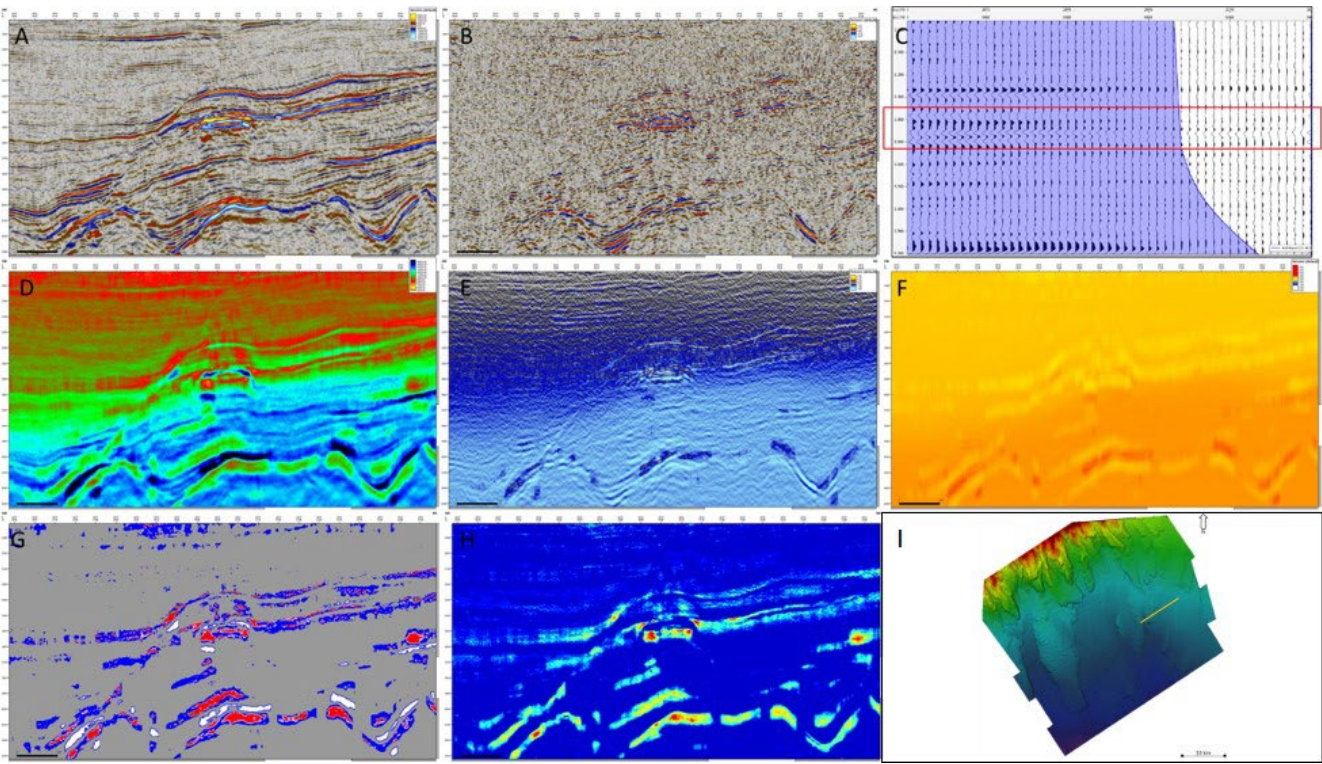
Figure 71: Cross-section along inline 2080 showing (A) KPSDM stack stretched to time, (B) AVA gradient, (C) gathers, (D) inverted P-impedance, (E) inverted V_p/V_s ratio (F) inverted density, (G) estimated lithology, (H) Hydrocarbon Probability and (I) location of seismic line
