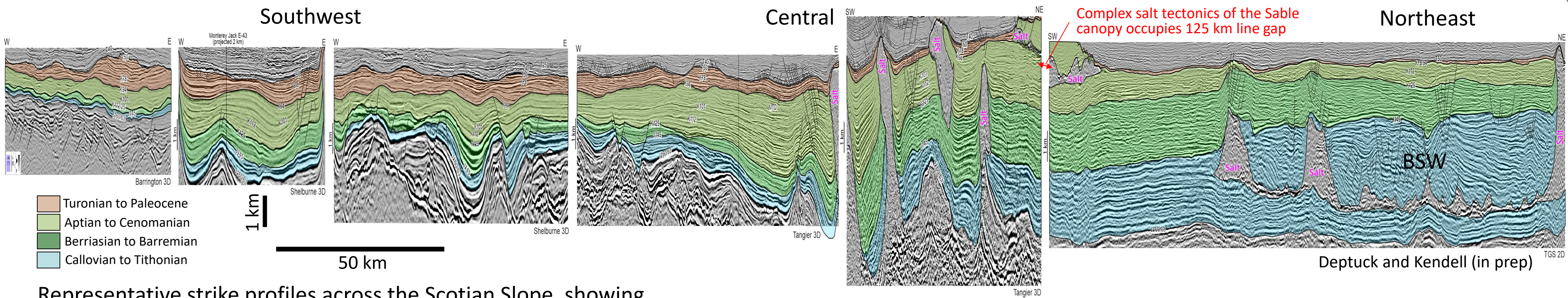
Representative strike profiles across the Scotian Slope, showing significant lateral variations in sediment thickness
