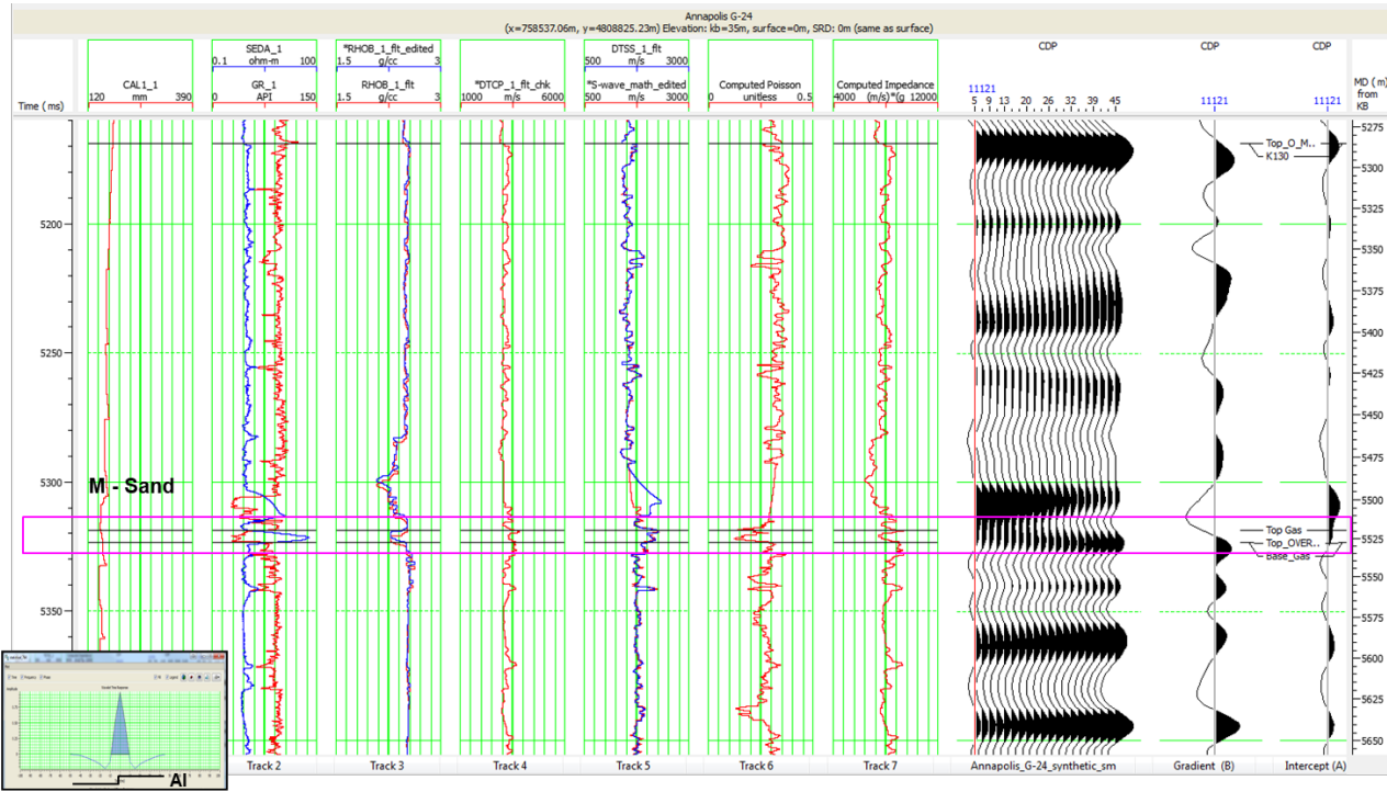
Figure 60: Angle Synthetic for Annapolis G-24 highlighting the M sand and top of gas (McQuaid and Hassan, 2013)
