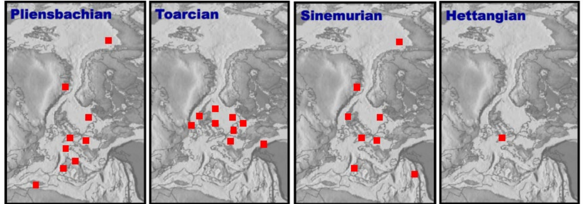
Figure 18: Distribution of significant organic rich sequences across the greater North Atlantic region, broken out by epoch. Locations per Figure . Lias (195 Ma) paleomap from Scotese (2014) (Bishop, 2020).
