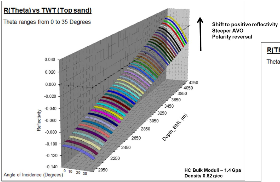
Figure 59: Forward model result at 1500m water depth for 80% Water Filled Cemented Sands (McQuaid and Hassan, 2013).
