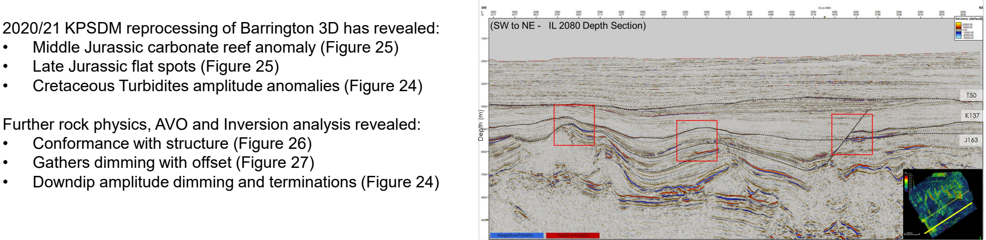
Figure 25: IL 2080 from the reprocessed survey highlighting 3 potential new leads (MacAdam et al. 2023).
