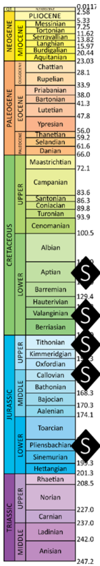
Figure 11: Five source rocks and their corresponding parameters modeled in the 2011 Play Fairway Analysis (Beicip et al.,2011).
