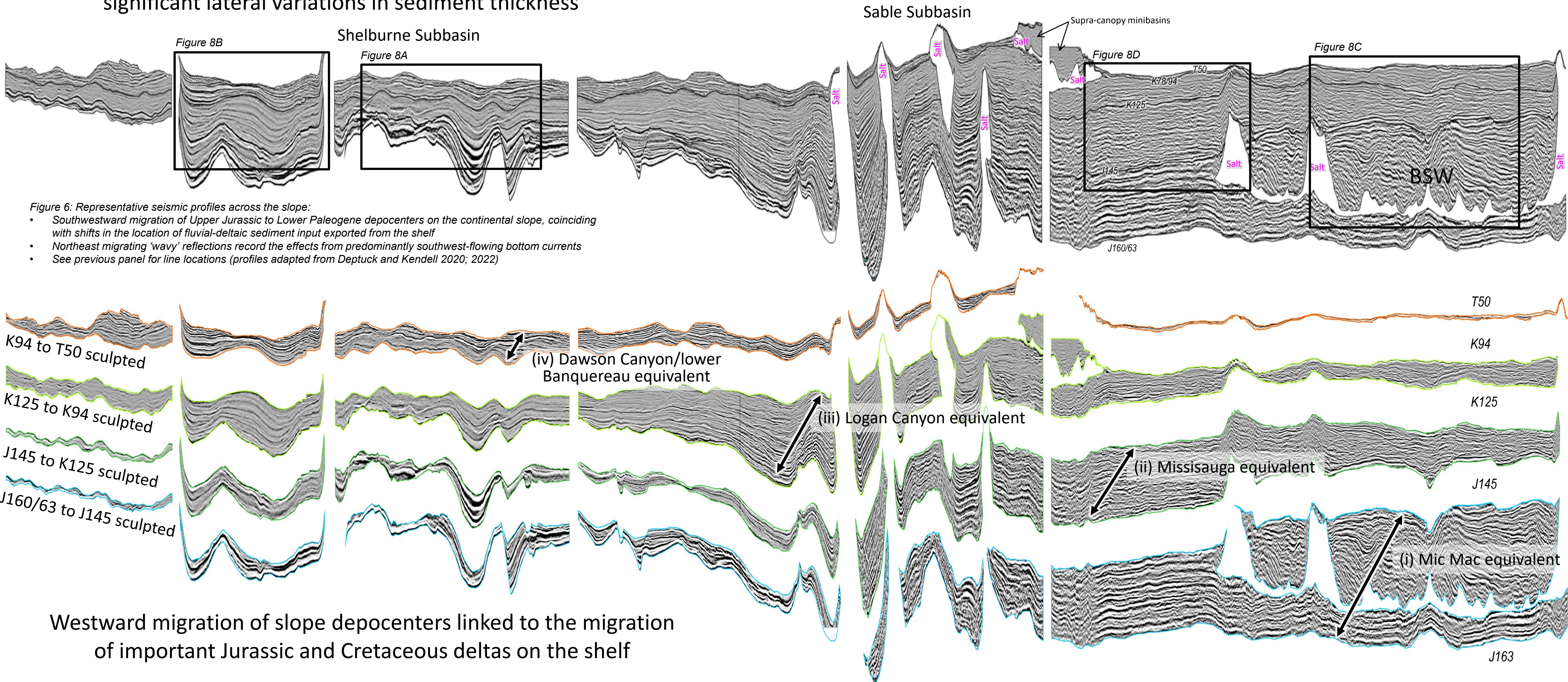
Representative strike profiles across the Scotian Slope, showing significant lateral variations in sediment thickness
