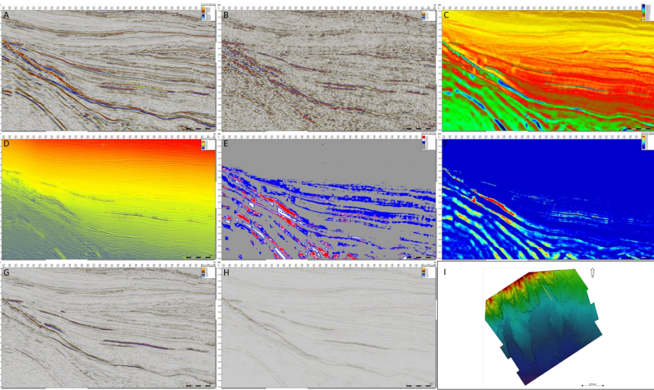
Figure 73: Cross-section along Xline 4800 showing (A) KPSDM stack stretched to time, (B) AVA gradient, (C) inverted P-impedance, (D) inverted VP/VS ratio, (E) estimated lithology, (F) Hydrocarbon Probability, (G) Near stack, (H) Far stack, and (I) location of seismic line
