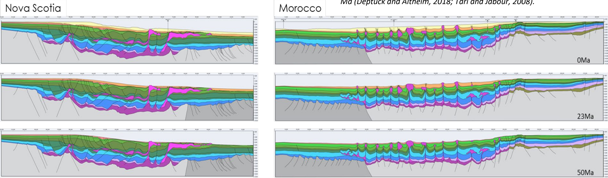
Figure 15: Examples of the conjugate margin reconstruction of Transect 2 from 0 to 50 Ma (NRR, 2020).
