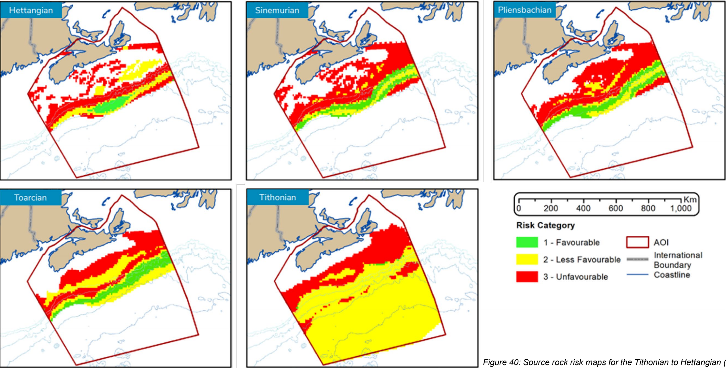
Figure 40: Source rock risk maps for the Tithonian to Hettangian (Scougal et al., 2021).
