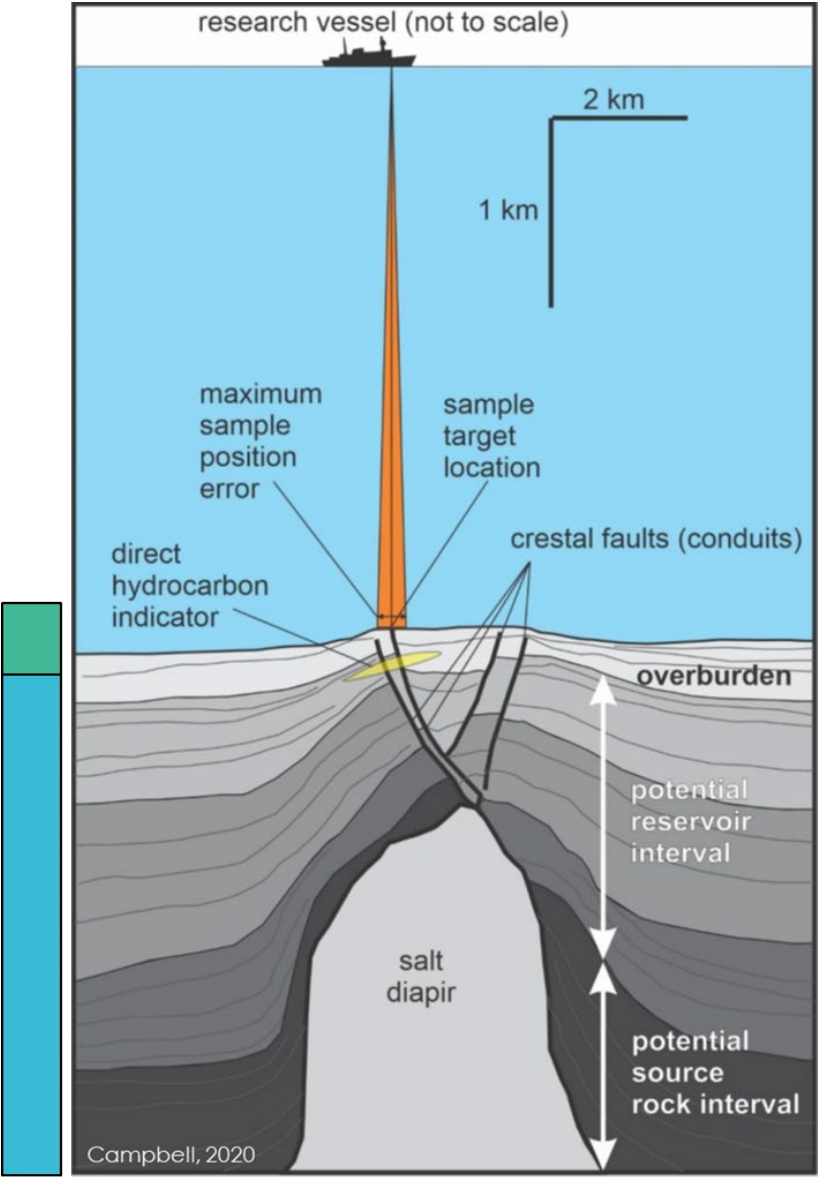
Figure 29: Diagram indicating an example of a piston coring target and potential error in coring location. Green bar represents depth of surface indication methods and blue the subsurface efforts (Campbell, 2020).
