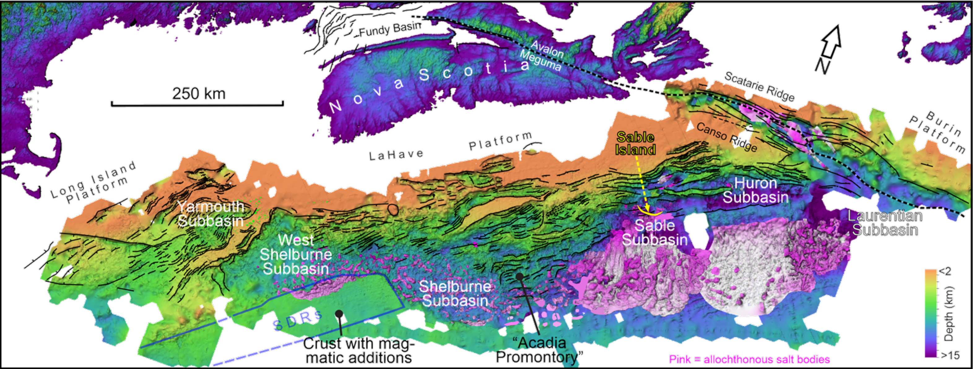
Figure 1: Study area in relation to the top basement structure map (lower) and the modern seabed (upper).
