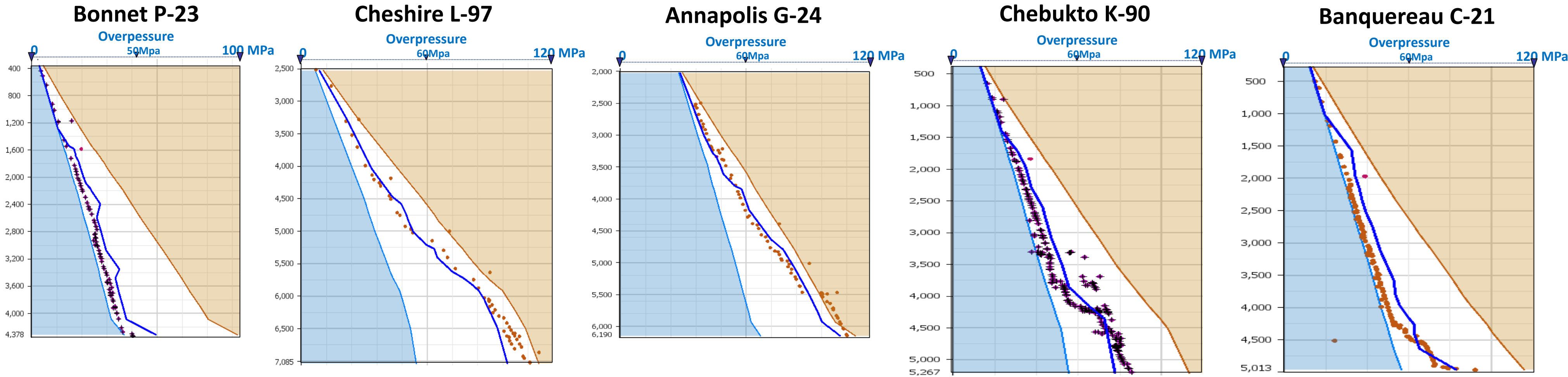
Figure 22: Pore-Pressure calibration
