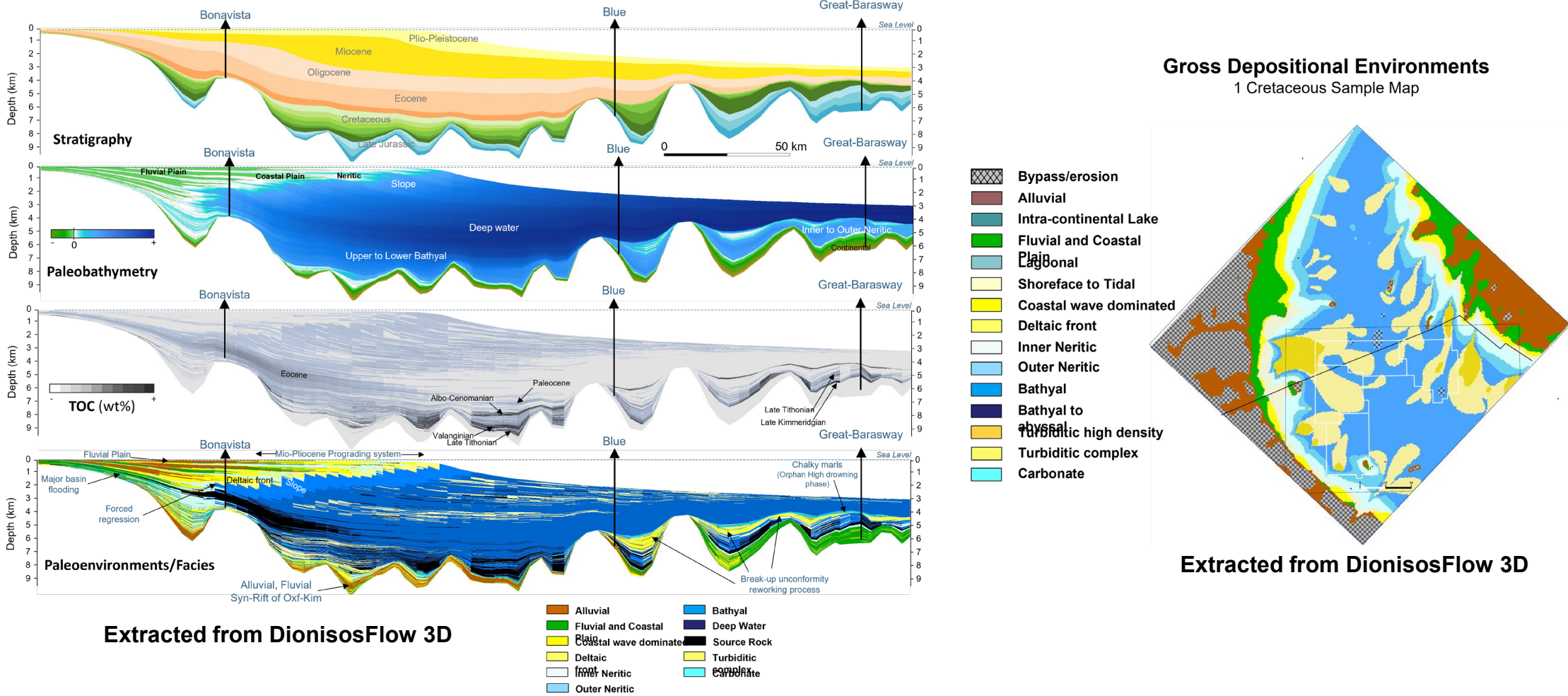
Figure 33: Example of DionisosFlow model from rifting to present day showing stratigraphy, paleo-bathymetry, lithofacies and organic matter content (Offshore Newfoundland & Labrador Resource assessment; Orphan Basin Area NL22-CFB01)
