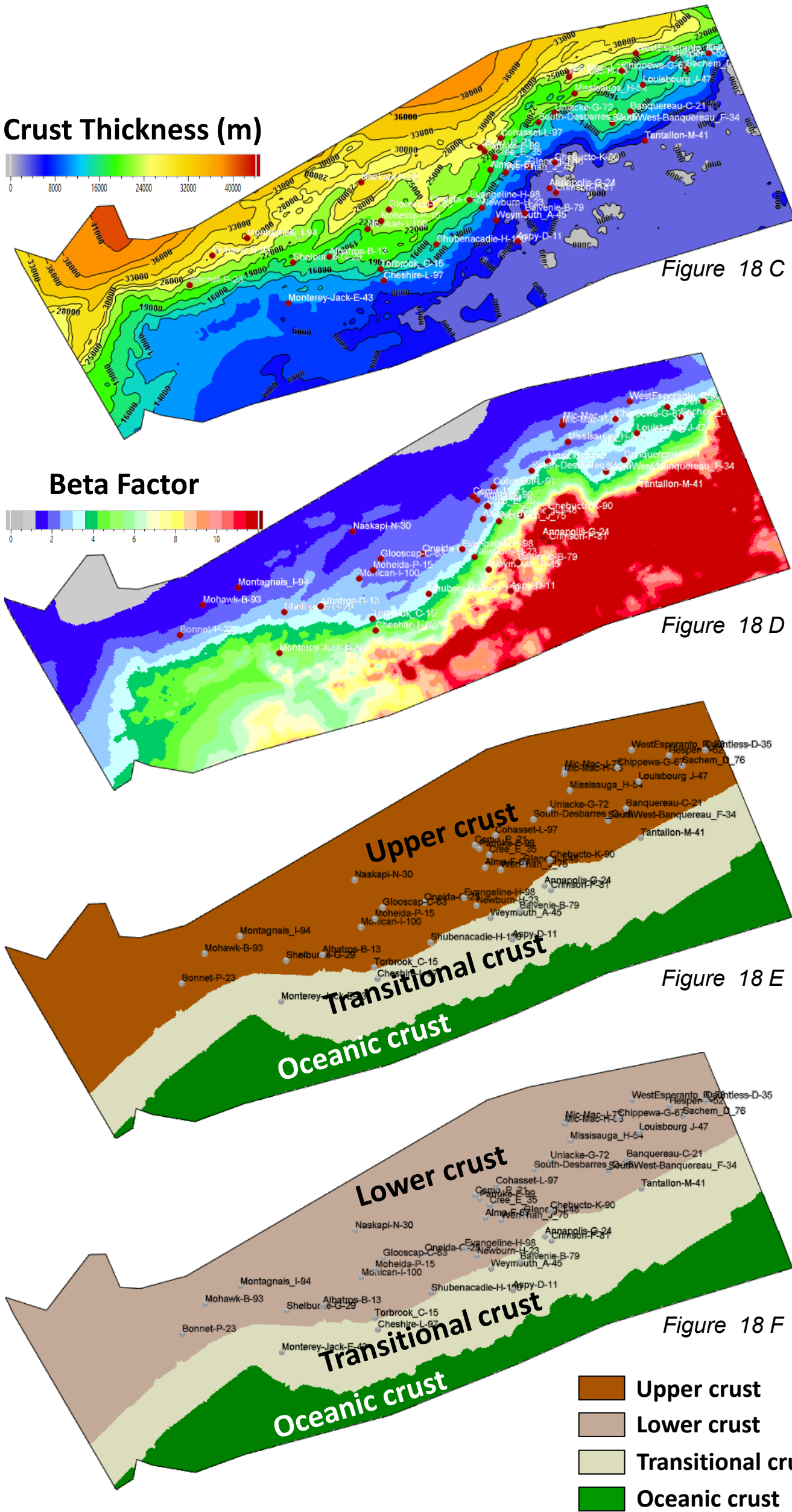
Figure 18: Maps used to build the lithospheric model (A, B, C, D, E and F)
