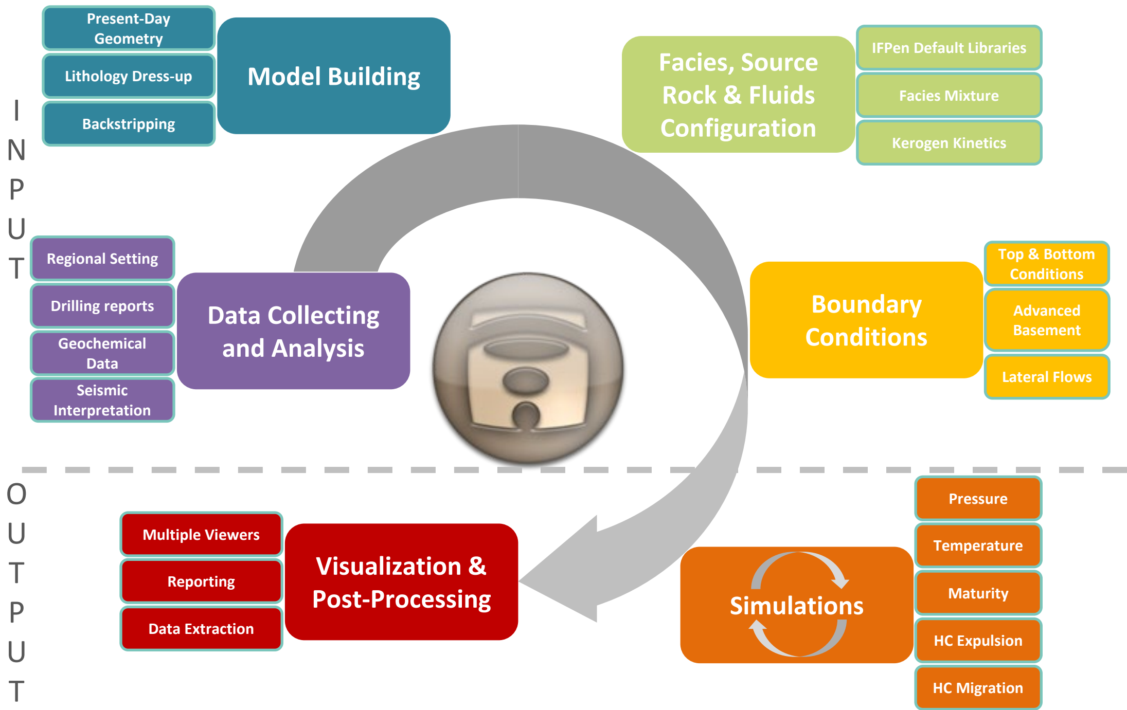
Figure 2: Basin Modeling workflow
