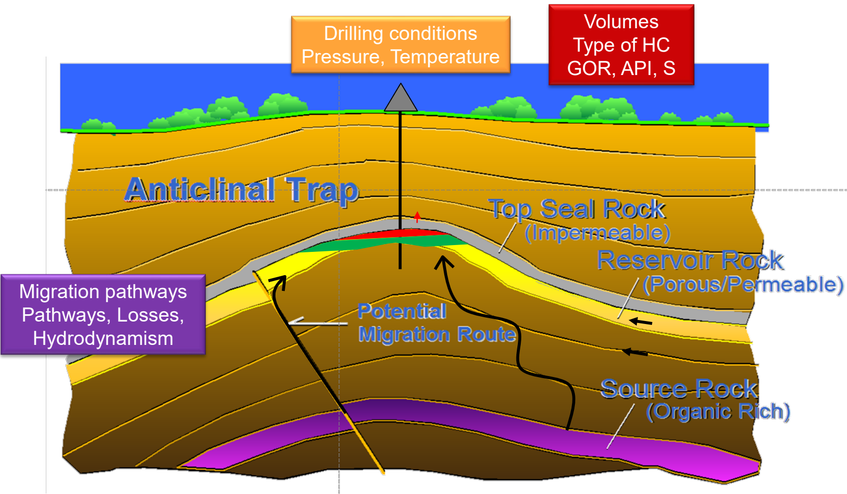
Figure 1: Principle of Petroleum System Model
