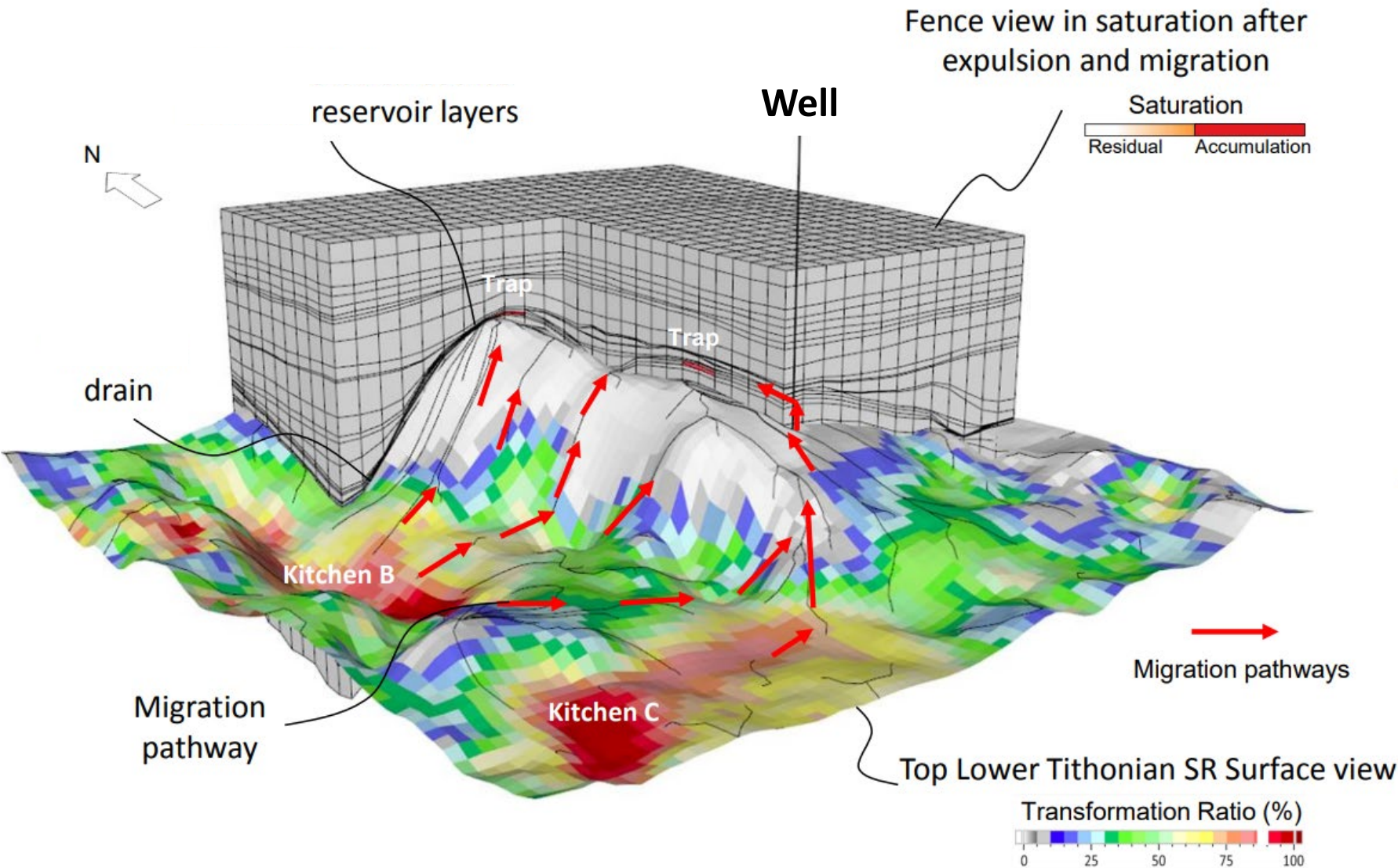
Figure 3: Example of Basin Modeling result
