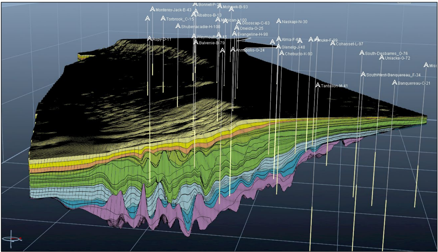
Figure 7: 3D view of Temisflow model displaying stratigraphy
