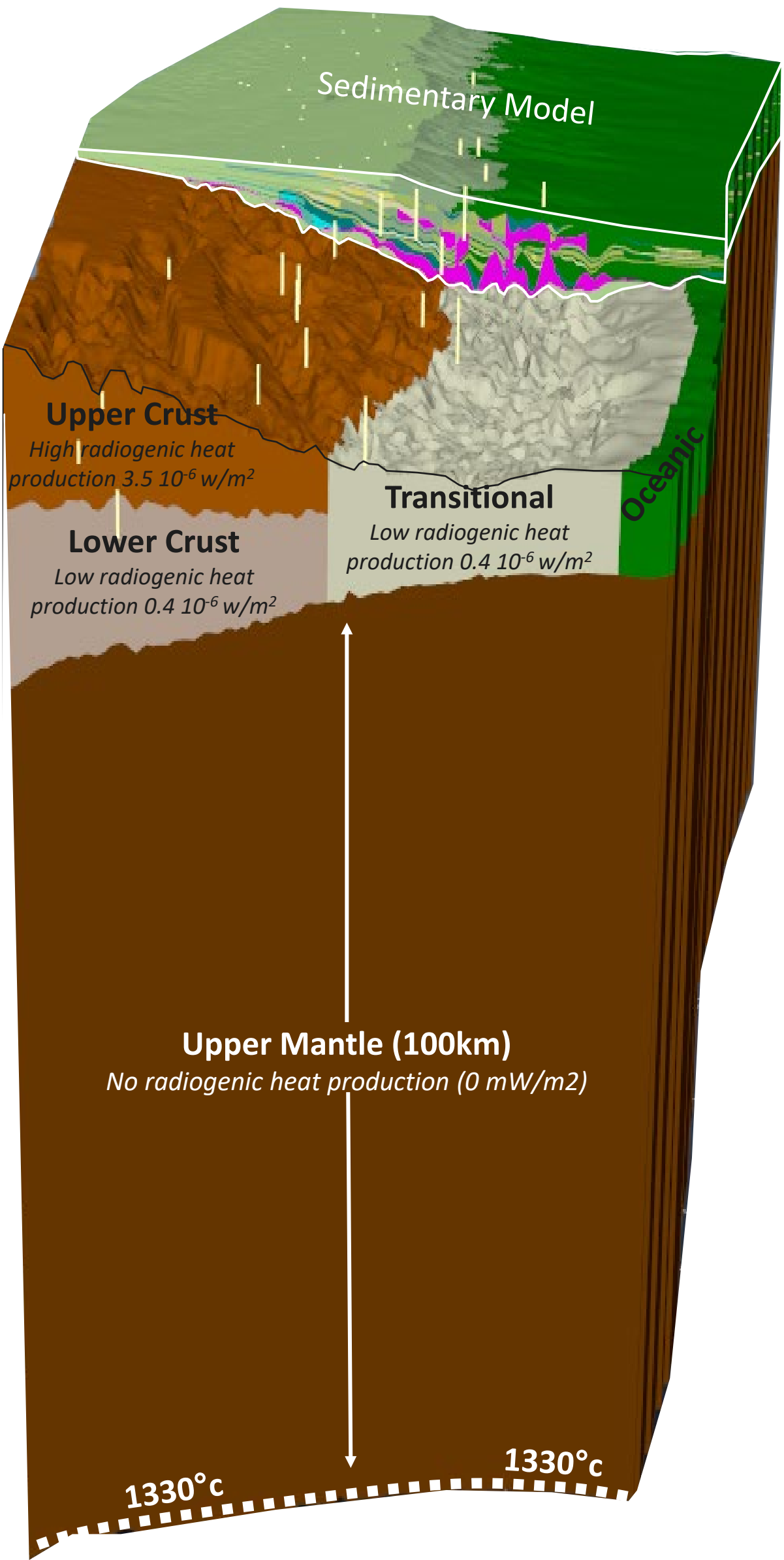
Figure 19: 3D view of the lithospheric and sedimentary model
