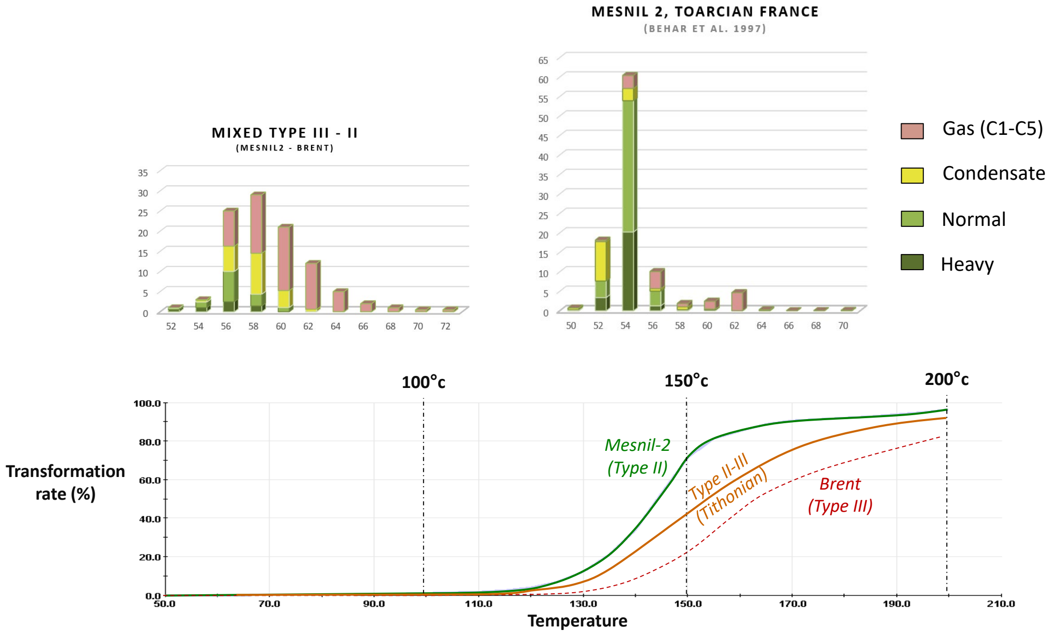
Figure 15: Kinetic scheme selected for the Tithonian and Pliensbachian source rocks
