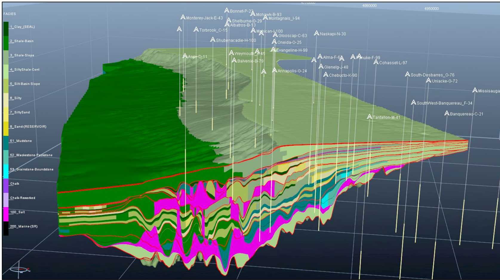
Figure 8: 3D view of Temisflow model displaying lithofacies
