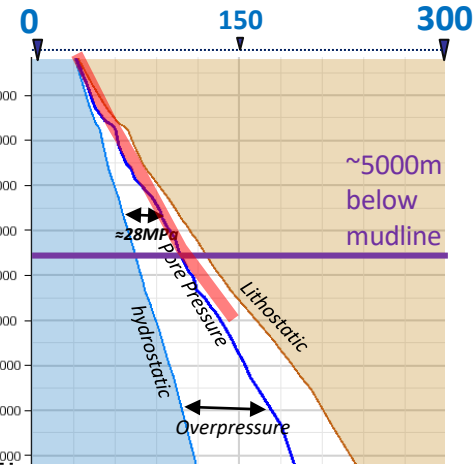
Pore Pressure (MPa) from Basin modeling at Seawolf lead location
