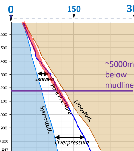
Pore Pressure (MPa) from Basin modeling at Piscatiqui lead location
