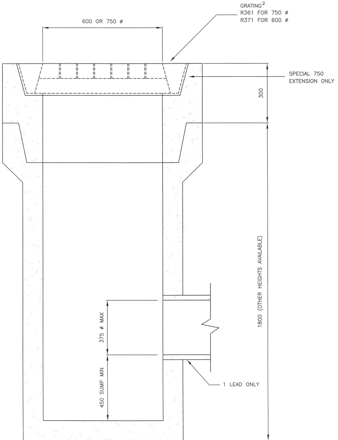
SECTION VIEW
