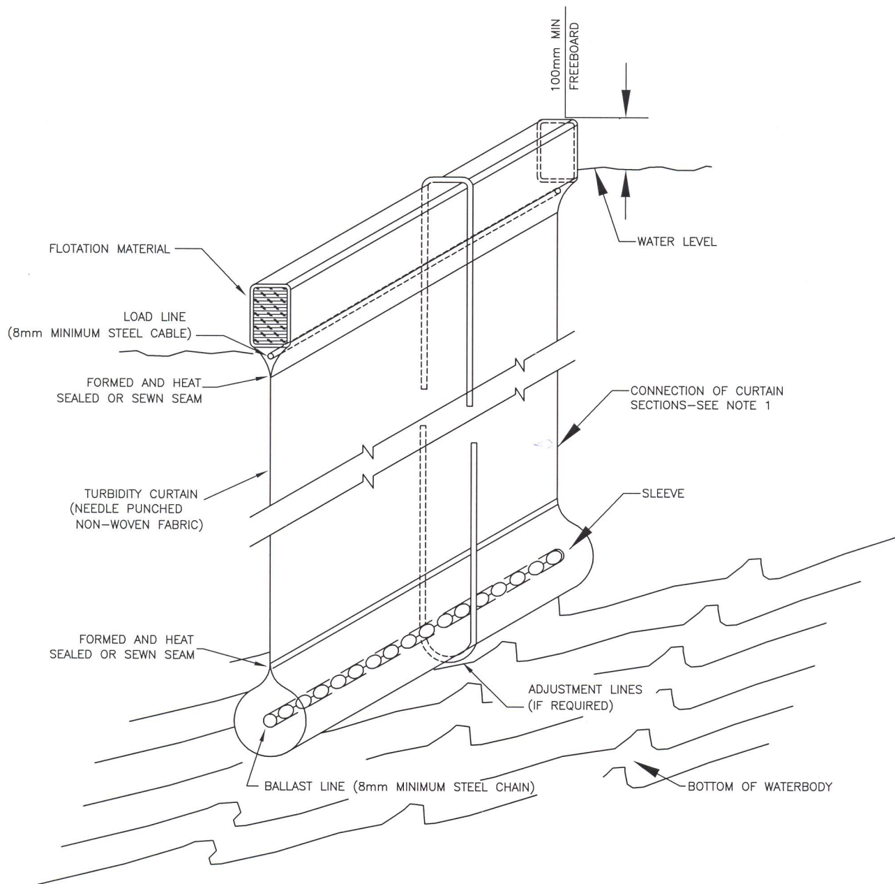
OBLIQUE VIEW
