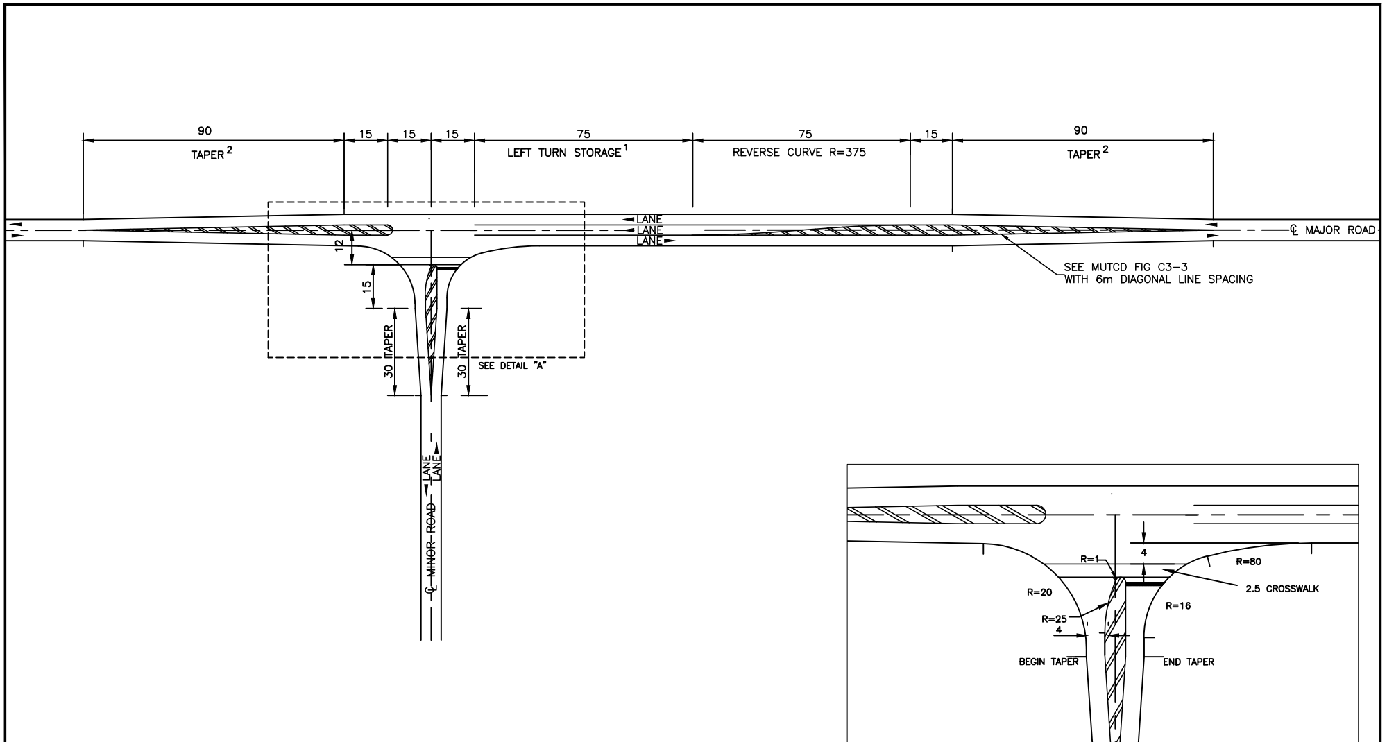
DETAIL "A"
